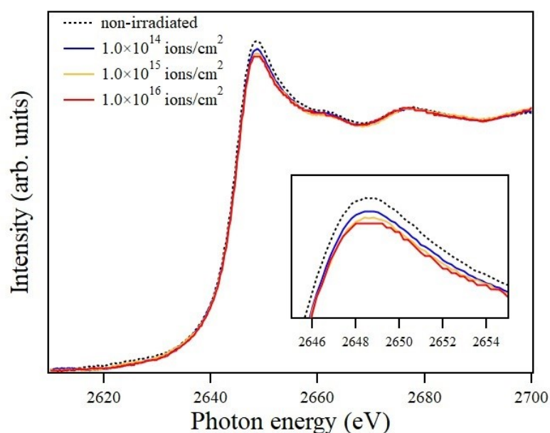
Fig. 3.11: XAFS spectra of Pt nanoparticles on the \text{Ar}^+ -irradiated glassy carbon substrates. The normalized XAFS spectra of the Pt M_3 -edge measured in the TEY mode using the BL-27A of the KEK-PF. The inset shows an enlarged view of the whiteline peaks. This figure is obtained by modifying Fig. 3 (a) of the preprint, T. Kimata et al., ChemRxiv. Preprint. (2017).
