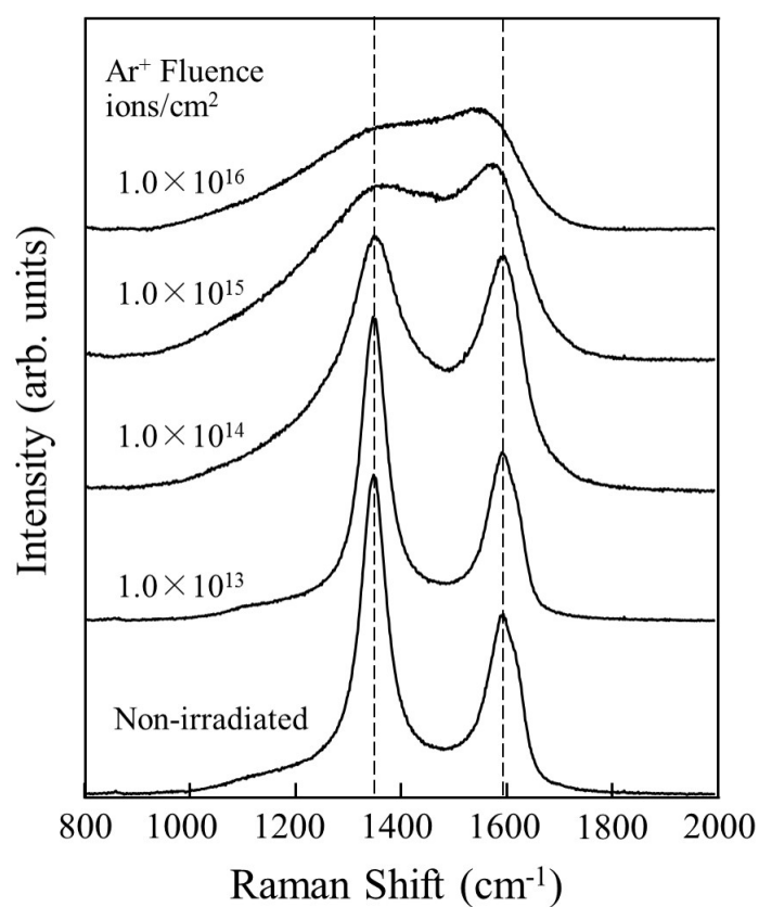
Fig. 4.3: Raman spectra of glassy carbon substrate irradiated at room temperature with 380 keV Ar + and then heated at 400°C in an N 2 atmosphere for 1 h. This figure is obtained from Fig. 1 of the paper, T. Kimata et al., Surf. Coat. Technol. 306, 123 (2016).
