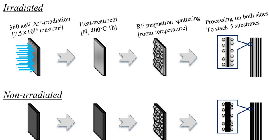
Fig. 3.12: Sample preparation schematic for the Pt L 3 -edge XAFS measurements at SPring-8. The glassy carbon substrates were irradiated with 380 keV Ar + at the fluence of 7.5 \times 10^{15} ions/cm 2 , and heated at 400°C in an N 2 atmosphere for 1 h. Pt nanoparticles were then deposited on the surface by rf magnetron sputtering for 60 s. This processing was treated both side of glassy carbon substrates, 5 substrates were stacked. This figure is obtained by modifying Fig. S6 of the preprint, T. Kimata et al., ChemRxiv. Preprint (2017).
