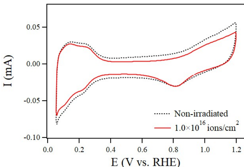
Fig. 2.4: Pt nanoparticles on the glassy carbon substrates irradiated with Ar ions as oxygen reduction catalysts. CV curves for Pt nanoparticles on the Ar + -irradiated glassy carbon substrates in an N 2 -saturated 0.1 M HClO 4 solution at a scan rate of 50 mV/s. This figure is obtained by modifying Fig. 1 (a) of the preprint, T. Kimata et al., ChemRxiv. Preprint. (2017).
