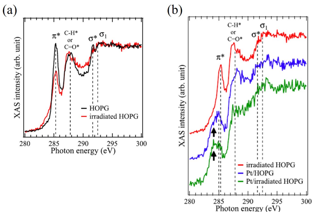
Fig. 3.18: (a) XANES spectra of the C K-edge for non-irradiated HOPG and \text{Ar}^+ -irradiated HOPG, measured at 30^\circ . (b) XANES spectra of \text{Ar}^+ -irradiated HOPG, Pt/non-irradiated HOPG, and Pt/ \text{Ar}^+ -irradiated HOPG measured at 30^\circ . Each spectrum is shown shifted in the y-axis direction. These figures are obtained by modifying Fig. 1, 2 of the paper, H. Okazaki et al., J. Chem. Phys. 152, 124708 (2020).
