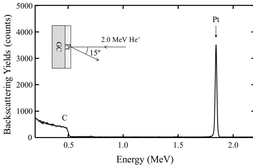
Fig. 3.7: RBS spectrum of the Pt nanoparticle layer on the non-irradiated glassy carbon substrate, measured with 2.0 MeV He + at 165°. This figure is obtained by modifying Fig. 2 of the paper, T. Kimata et al., Surf. Coat. Technol. 306, 123 (2016).
