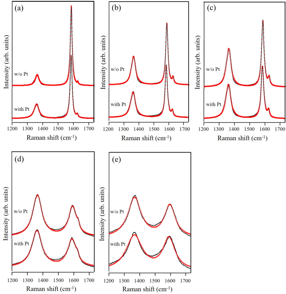
Fig. 4.11: The Raman spectra of the HOPG irradiated with Ar + at a fluence between 1.0 \times 10^{12} and 1.0 \times 10^{14} ions/cm 2 without and with Pt deposition. These figures are obtained by modifying Fig. 3 of the paper, T. Kimata et al., Nucl. Instrum. Meth. Phys. Res. B 444, 6 (2019).
