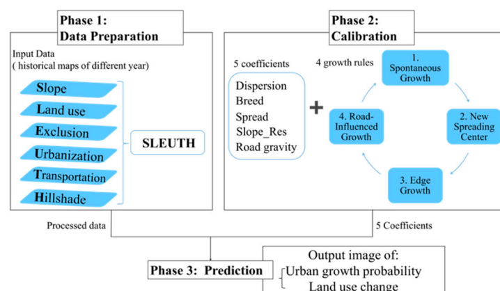
Figure 1. SLEUTH model structure (Source: based on Dietzel and Clarke, 2004 [7]; Clarke and Hoppen, 1997 [8]).
