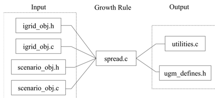
Figure 6. Summary of modifications in source code.
