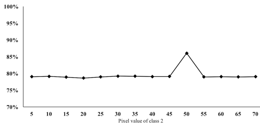
Figure 9. Accuracy (vertical axis) of Extended SLEUTH when changing pixel value of class 2 (non-station and non-water area) from 5 to 70 (horizontal axis). The horizontal axis represents case runs of Extended SLEUTH, where each case represents variations in the representative values of class 2 (e.g., 5 means that an Extended SLEUTH run with all pixels in the exclusion layer representing class 2 were set to 5).
