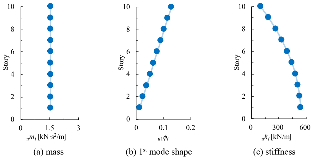
Fig. 2 – Structural properties of the upper structure
