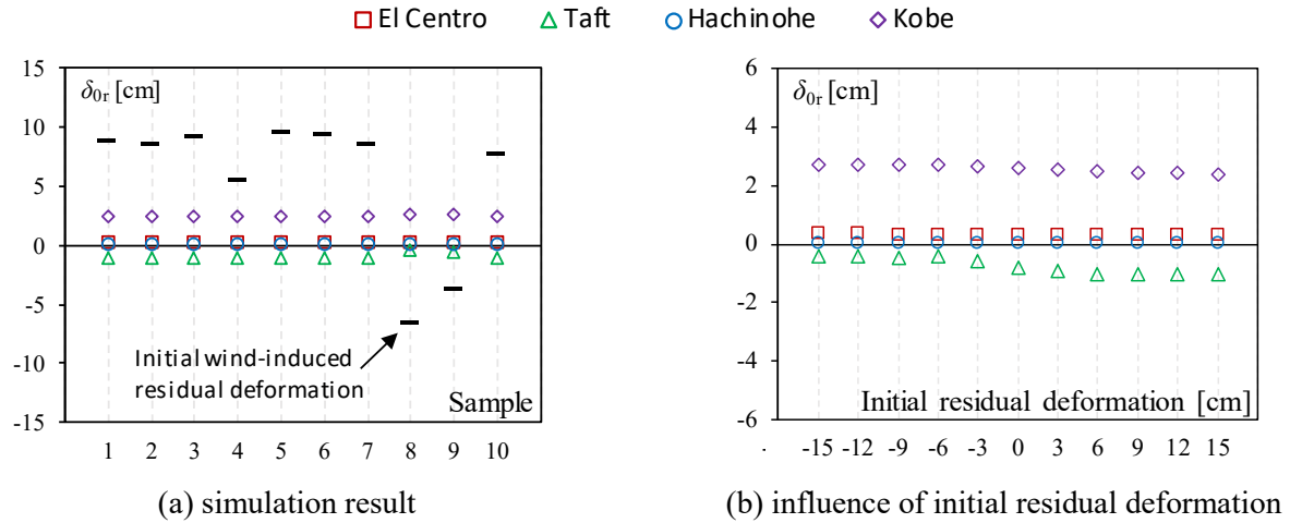
Fig. 7 –Residual deformation in the isolation story (NS)
