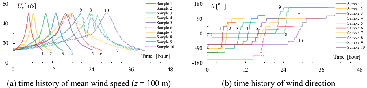
Fig. 4 – 10 assumed typhoon samples in the typhoon simulation
