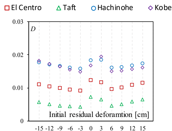
Fig. 12 –Influence of initial residual deformation on D value (NS)
