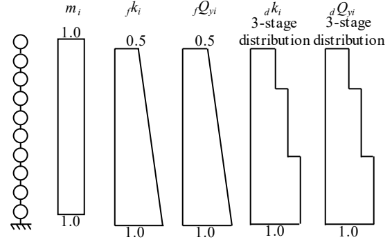
Fig. 3 Analysis model
