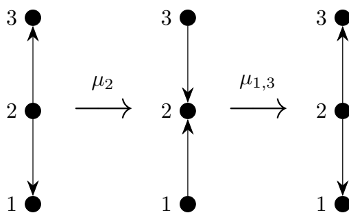
Fig. 3.4 The mutation loop for type (A_1, 4) .
