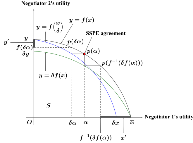
Figure 3.9: SSPE agreement at period 2
