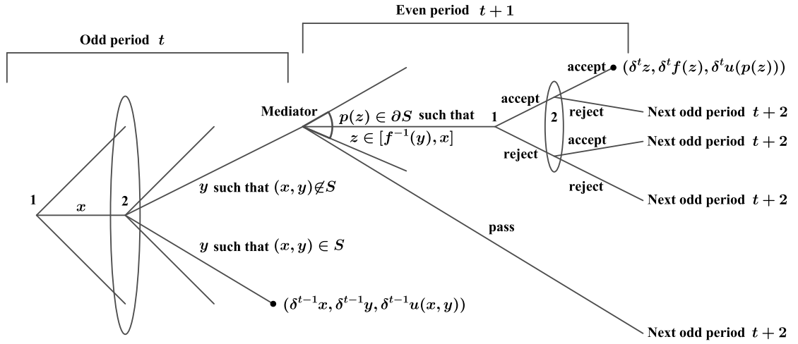
Figure 3.3: Game tree
