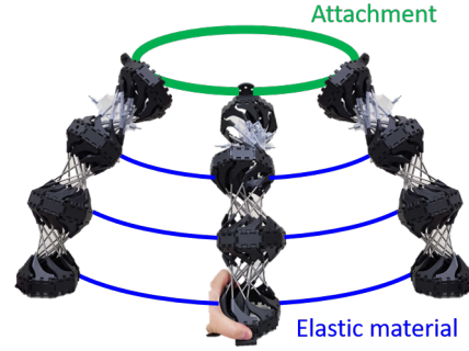
Figure 6.2: Extendable mechanisms placed in parallel following the concept in Fig. 1.6
