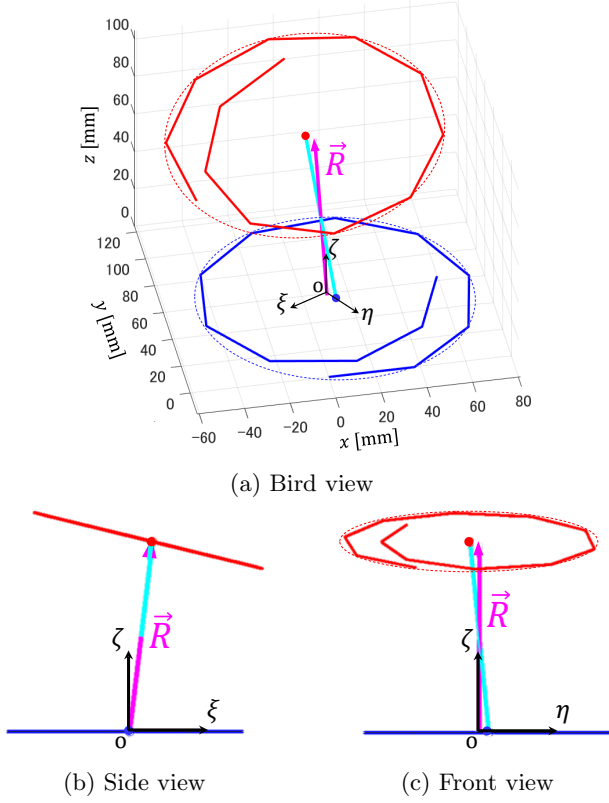
Figure 3.14: Relative position vector \vec{R} in Origami Spring
