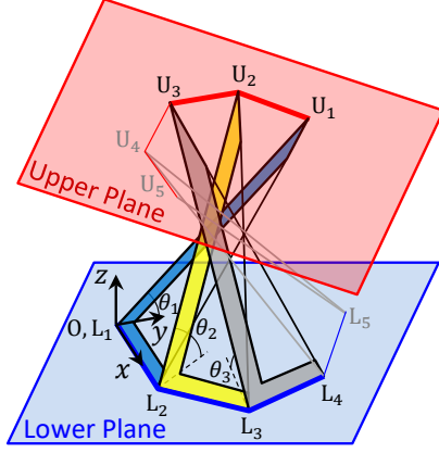
Figure 3.6: Independent variables of Origami Spring
