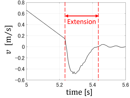
Figure 5.17: Example of time change of velocity during the extension motion. The steady state of velocity after extension is set as 0. The end of extension is when v becomes 0 after the extension.
