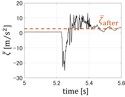
Figure 5.16: Example of change of acceleration \ddot{\zeta} during the extension motion. Acceleration \ddot{\zeta} includes the acceleration of gravity and \ddot{\zeta}_{\text{after}} is the steady state after extension.
