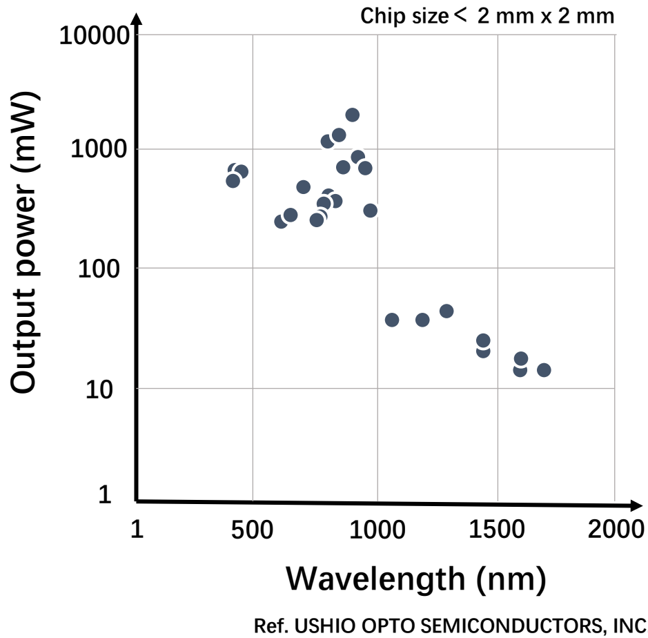
Fig. 2.19 Characteristics of output power of high-power LEDs in market
