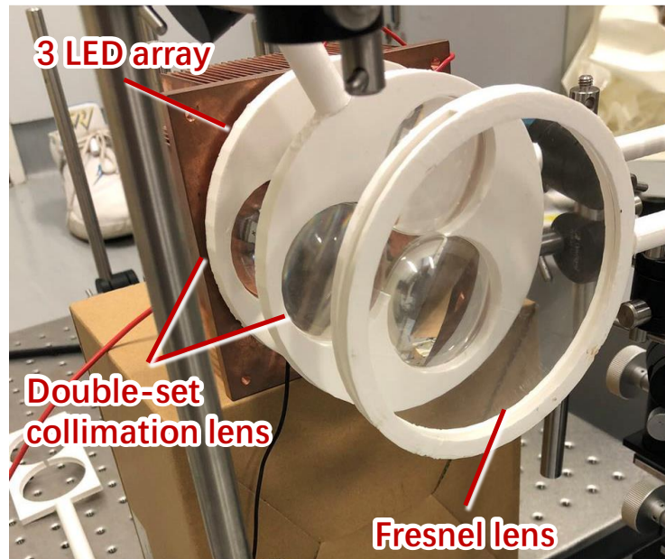
Fig. 5.13 The experiment setup of 2-LED array OWPT system (configuration B)
