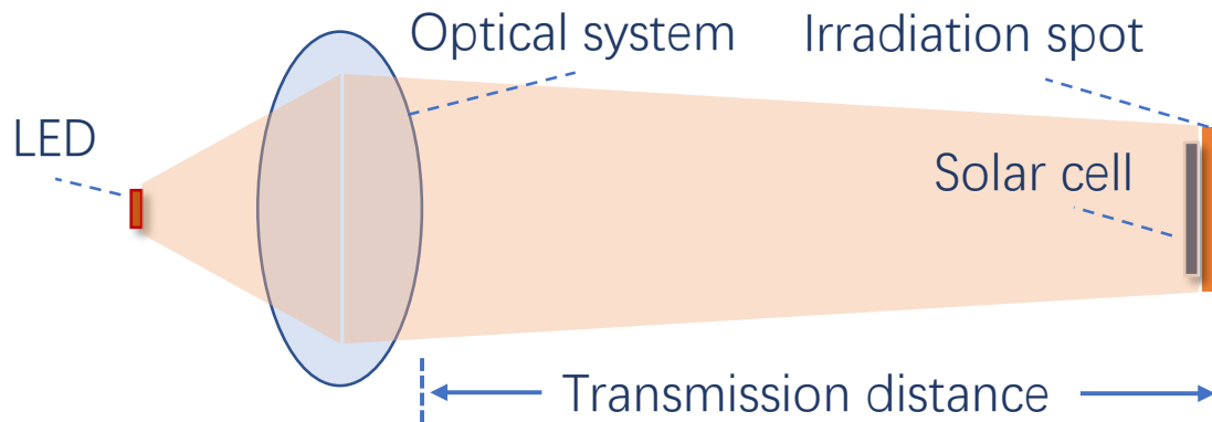
Fig. 2.3 The basic configuration of LED-based OWPT system
