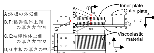
Fig. 1 Viscoelastic damper specimen with the temperature measurement locations
