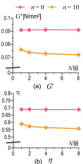
Fig. 8 Character due to N
