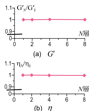
Fig. 7 Ratio of Static analysis
