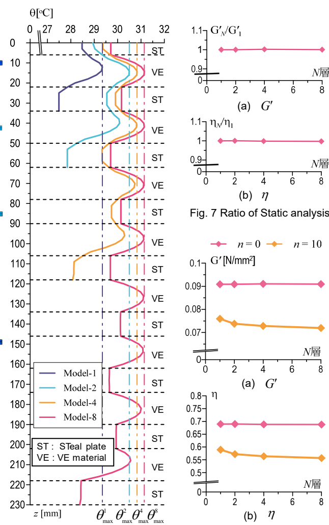
Fig. 6 Distribution of temperature
