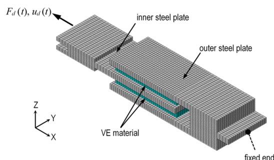
Fig. 2 3D - FEM model - Full VE damper
