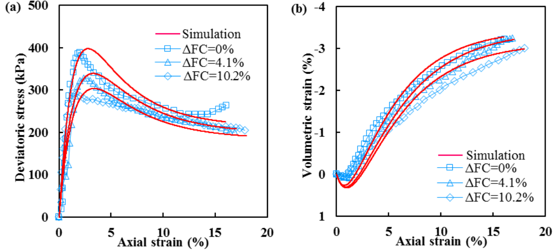
Fig. 5 Simulation results of drained triaxial compression tests after erosion through the modified model on dense soils. a stress-strain response, b volumetric strain-axial strain response (After Li et al., 2020)
