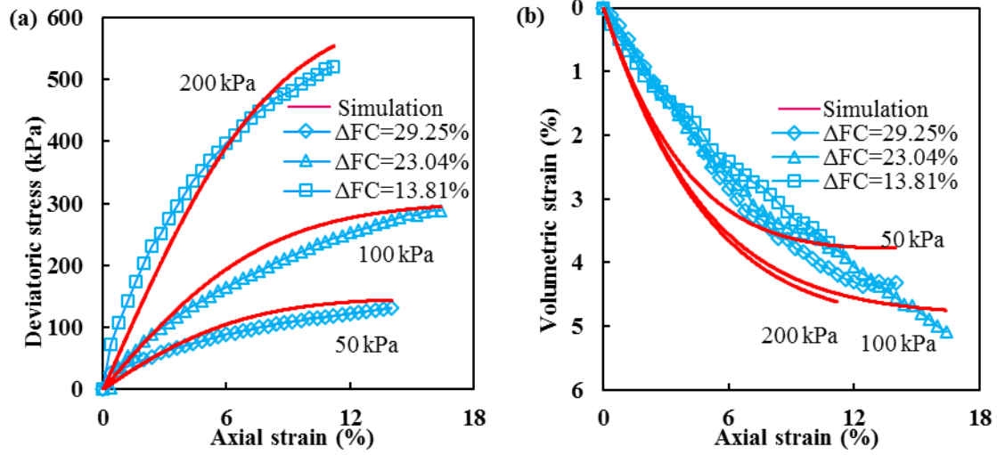
Fig. 3 Typical simulation results of drained triaxial compression after erosion through modified model on loose soils; (a) stress-strain response, (b) volumetric strain-axial strain response (After Ke and Takahashi, 2014)
