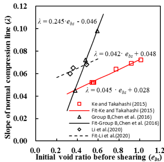
Fig. 8 Relationship between slope of normal compression line and initial void ratio before shearing
