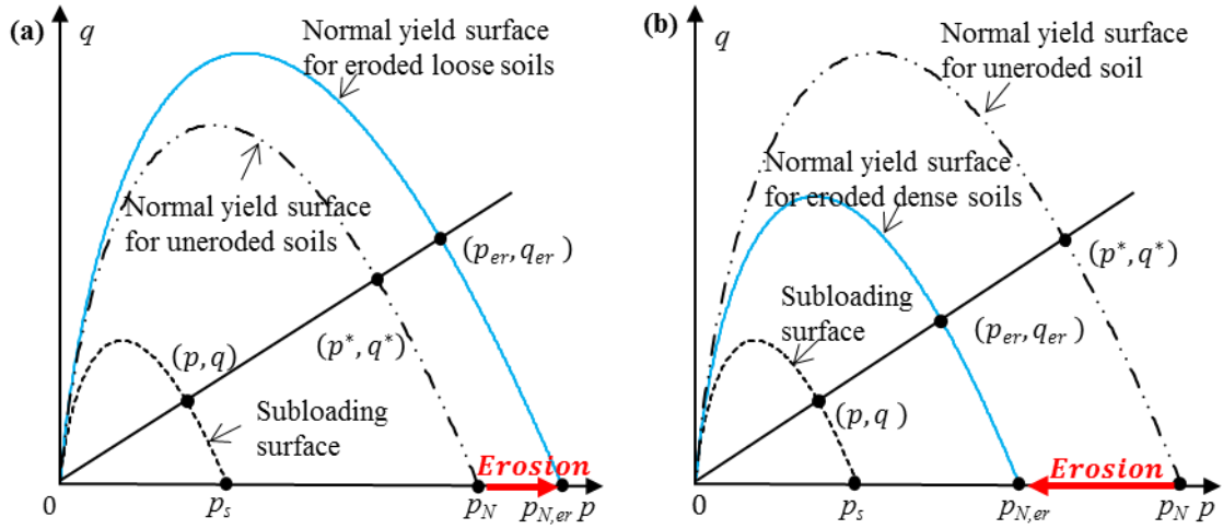
Fig. 2 Concept of normal yield surface for eroded soils. a loose soils, b dense soils
