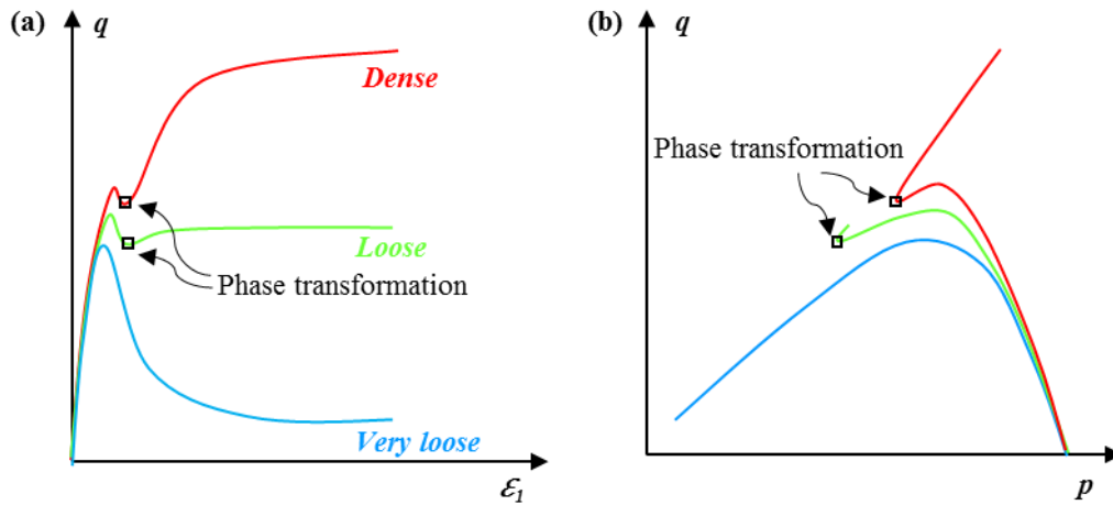
Fig. 14 Typical mechanical behaviour of sand under undrained condition and definition of phase transformation state; (a) deviatoric stress-axial strain response, (b) effective stress path
