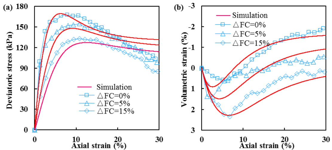
Fig. 12 Comparison between experimental and simulation results of drained triaxial compression after erosion on dense soils (Group A, Chen et al., 2016); (a) stress-strain response, (b) volumetric strain-axial strain response
