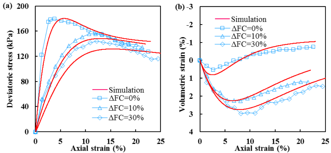
Fig. 4 Simulation results of drained triaxial compression tests after erosion through modified model on dense soils (Group B); (a) stress-strain response, (b) volumetric strain-axial strain response (After Chen et al., 2016)
