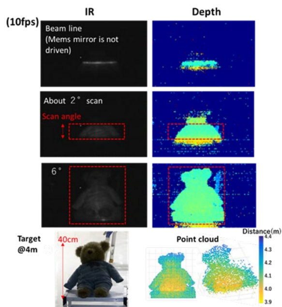
Fig. 1 Example image of Real-time LiDAR measurement
