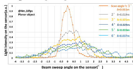
Fig. 2 Light intensity and accuracy of each scan range
