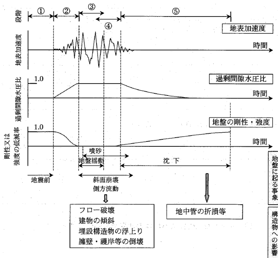
Figure 2.3.2 Conceptual diagram of ground behavior due to liquefaction during earthquake (Sasaki, Moriwaki and Ohbayashi, 1997)
