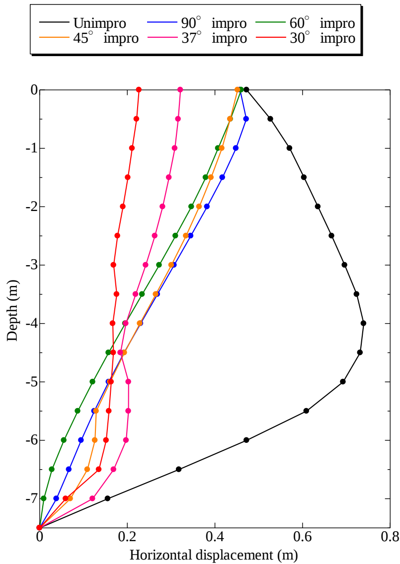
Figure 5.3.7 Distribution of horizontal displacement under embankment toe ( t = 50\text{ s} )
