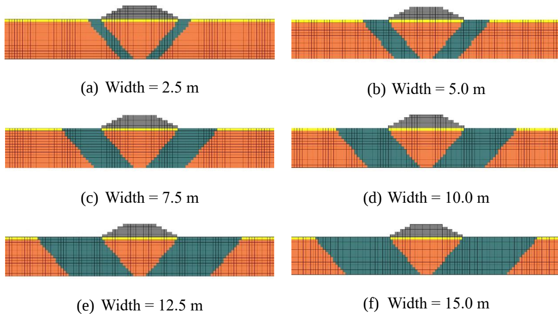
Figure 6.2.1 Discretized mesh for the 2D FE analysis models
