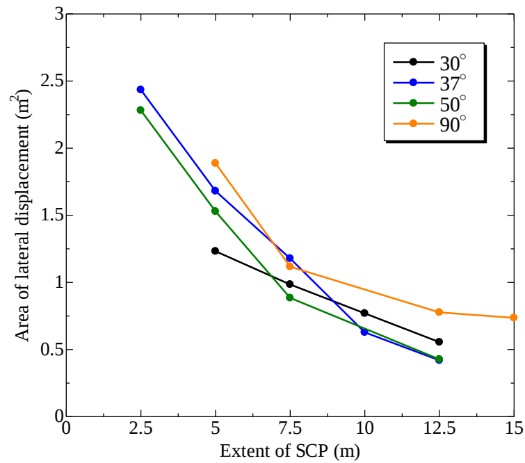
Figure 6.3.4 Relation between extent of SCP and Area of lateral displacement
