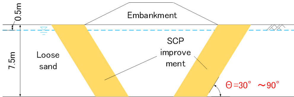
Figure 5.1.1 Schematic of FE analysis model
