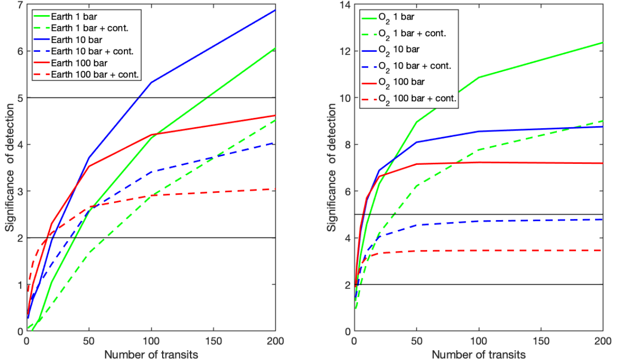
Figure 3.33: Left: Number of transits of TRAPPIST-1e required to reach a 5- \sigma detection in an Earth-like atmosphere for different pressures with continuum processes (dashed lines) and without the continuum processes (solid lines). Right: Similar plots for desiccated O 2 atmospheres. Black horizontal lines in both panels mark the 2- \sigma and 5- \sigma detection levels.
