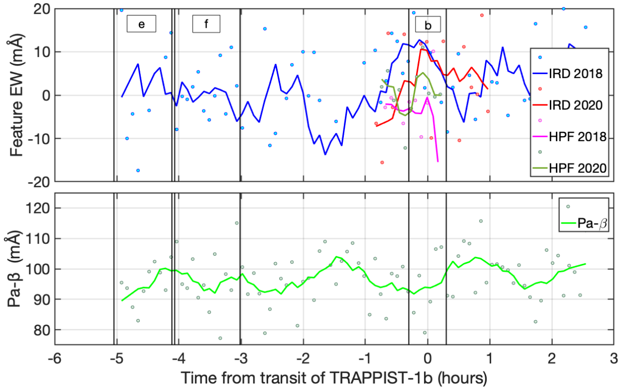
Figure 3.9: Top: Strength of the feature between 1083.285 and 1083.34 nm (“region of interest”) vs. time as measured in IRD (UT 30 August 2018 - blue and UT 2020 September 16 - red) and HPF (UT 2018 October 2 - magenta and UT 2020 September 5 - green) spectra. The solid lines represent 7-point, first-order Savitzky-Golay filtered versions. Bottom: EW of Hydrogen Paschen beta line as measured in IRD spectra on UT 30 August 2018. Both panels correlates negatively.
