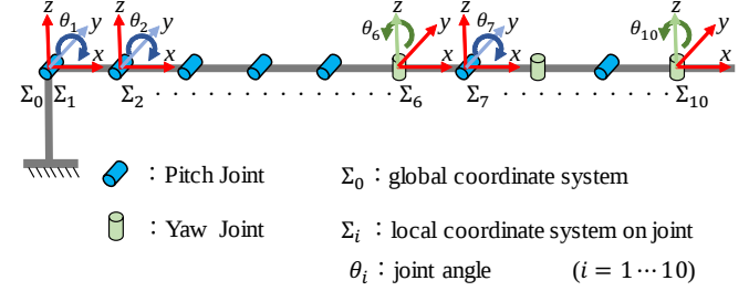
Fig. 3. Kinematically redundant joint configuration of Super Dragon.
