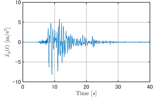
(a) Accelerogram
