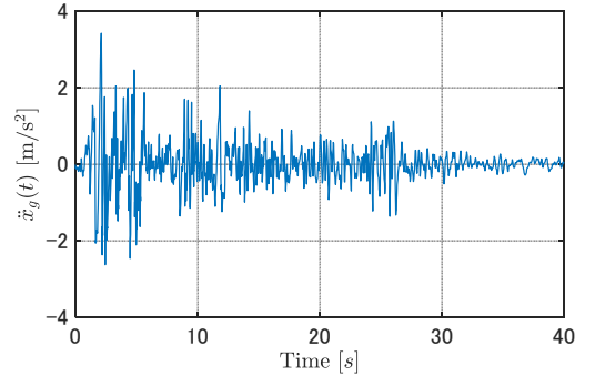
(a) Accelerogram
