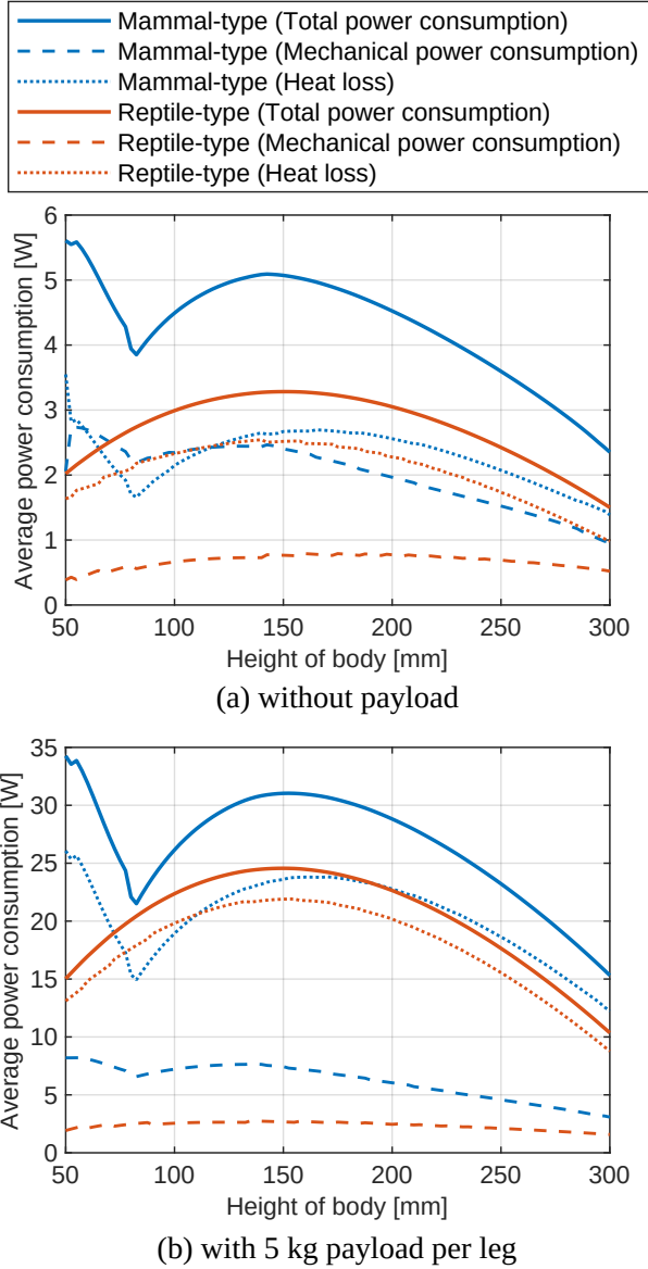
Fig. 12. Relationship between body height and average power consumption for the trajectory that minimizes energy consumption per step.
