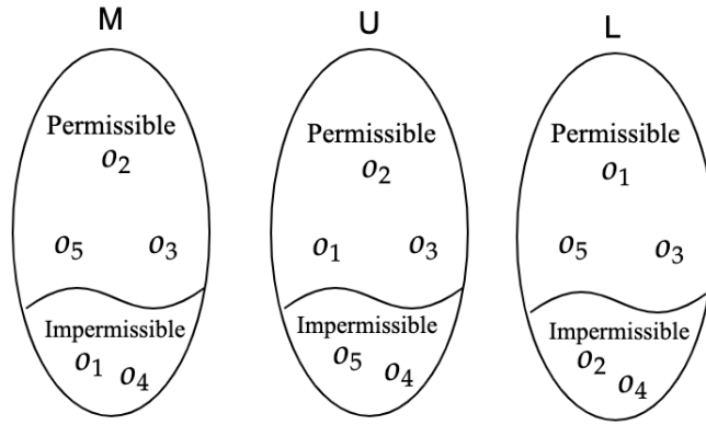
FIGURE 6.3: Elmira-Option PR: OP_M^{2\backslash iv} , OP_U^{2\backslash iv} , OP_L^{2\backslash iv}
