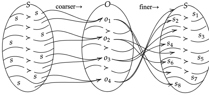
FIGURE 4.1: Coarsening and Refinement of information - GMCR DA
