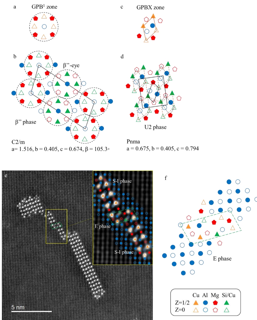
Fig. 3.10. Atomic models (a-d, f) and HAADF-STEM image (e) of selected precipitates. (a) GPB 1 zone, (b) \beta'' phase, (c) GPBX zone, (d) U2 phase, and (f) E phase. (e) HAADF-STEM image of S-I and E phases in the AR sample aged at 443 K for 1 day, with the partial atomic overlay.
