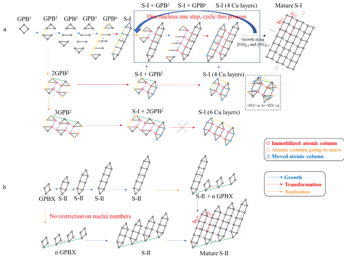
Fig. 3.8. Simplified schematics of the precipitation processes, showing the formation and growth of (a) S-I and (b) S-II phases in a \langle 100 \rangle_{Al} projection, in terms of the Cu-columns only. (a) The precipitation process from GPB^1 zone to mature S-I phase. (b) The precipitation process from GPBX zone to mature S-II phase.
