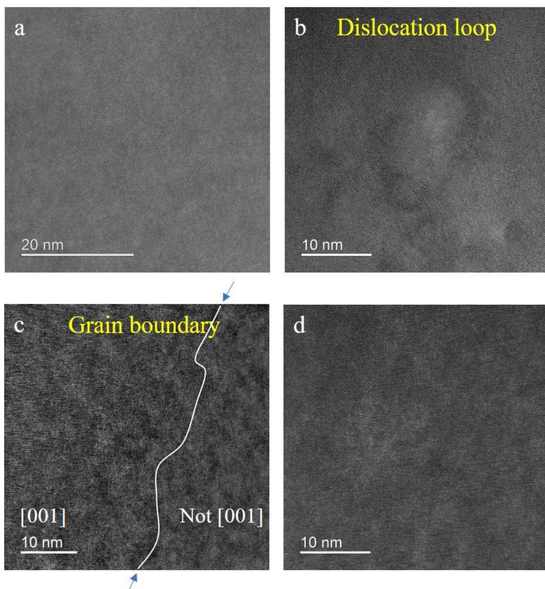
Fig. A.1. HAADF-STEM images of the as-quenched (AQ) and as-rolled (AR) samples, showing no precipitate has been formed. (a) The Al matrix in the AQ sample. (b) Example of quenched in dislocation loop in the AQ sample. (c) (FFT filtered image) Two grains in the AR sample, separated by blue arrowed grain boundary. The left side grain is orientated in a \langle 001 \rangle_{\text{Al}} direction, while the right side is different since no clear atomic arrangement cannot be found. (d) The Al matrix in the AR sample.
