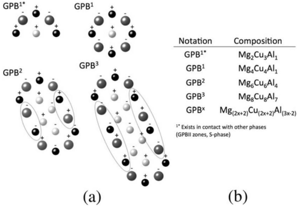
Fig. 1.6 (a) Structural relationship between the 1D-GPBx crystals. The 1D-GPBx are depicted along their periodic direction. The plus and minus signs indicate the position of the atoms along z in these 1D periodic cells: plus, z = 0.5 ; minus, z = 0 . (b) Stoichiometries of the 1D crystals of the GPB zones [39].
