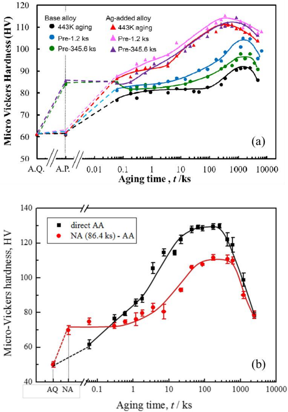
Fig. 1.8 (a) Two-step aging (pre-aging at 323 K) effects on the hardness for the Base (Al-Mg-Cu) and Ag-added (Al-Mg-Cu-Ag) alloys [46]. (b) Hardness changes for the Al-Mg-Si alloy during artificial aging at 443 K directly and two-step aging after natural aging at RT for 86.4 ks [48].
