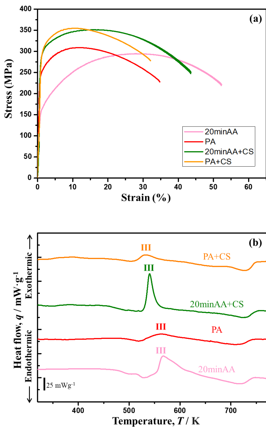
Fig. 4.4 (a) Engineering stress-strain curves and (b) DSC curves for the samples that were artificially aged for 20 min (20minAA), peak-aged (PA), artificially aged for 20 min then cyclically strengthened (20minAA+CS), peak-aged then cyclically strengthened (PA+CS).
