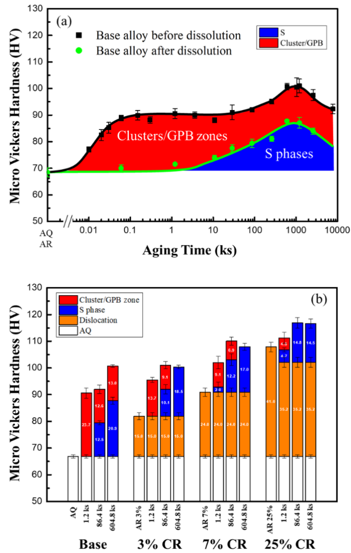
Fig. 2.6 (a) Hardness curves of aged base alloy before and after dissolution experiments. (b) Hardness contribution of dislocations and precipitates in both base and CR samples.
