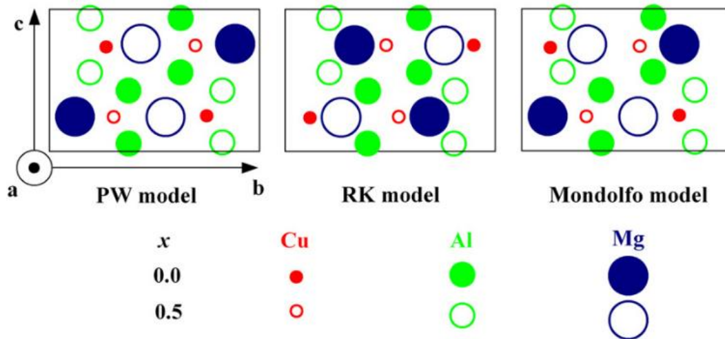
Fig. 1.7 Schematic unit cells of the existing controversial structure models for S-phase, projected along the [100]_S direction. a , b and c are the lattice vectors, and x is the fractional coordinates of atoms in the a or [100]_S direction. In the Mondolfo model, one of the (001)_S Cu–Mg atomic layers is shifted along [010]_S with respect to that in the PW model. The difference between the RK model and the PW model is that the Cu atoms and the Mg atoms are swapped [45].
