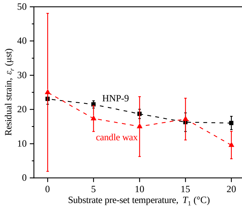
Fig. 3.11 Comparison of residual strains for candle wax and HNP-9 under each substrate pre-set temperature at drop heights of (a) 50 mm and (b) 100 mm when the droplet temperature was fixed at 140 ^{\circ}\text{C} .
