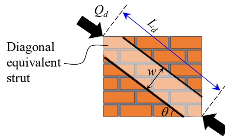
Fig. 3-40. Effective width of the diagonal strut.
