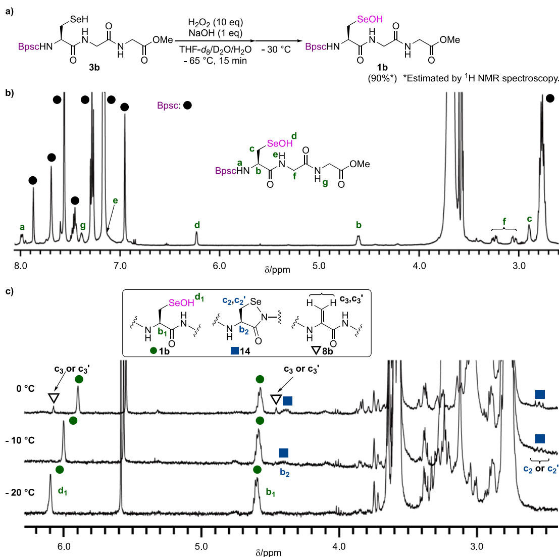
Figure 5. (a) Generation of 1b . (b) 1 H NMR spectrum (500 MHz) of 1b in THF-d 8 /D 2 O at -30 °C. (c) VT NMR spectra (400 MHz, -20 up to 0 °C) for a solution containing 1b in THF-d 8 /D 2 O.
