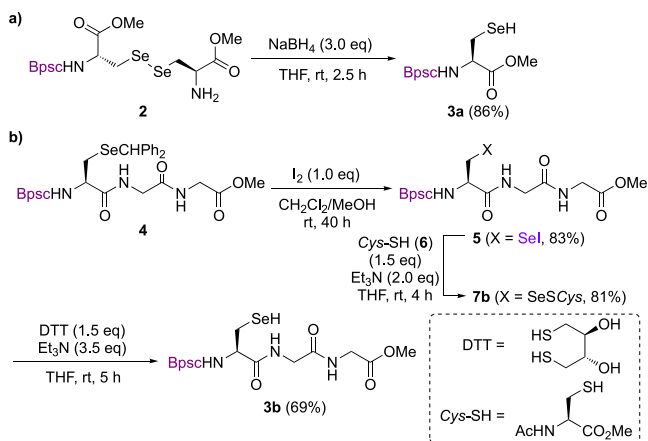
Scheme 1. Synthesis of the Selenols of the Sec Model (a) and the Sec-Gly-Gly Model (b)
