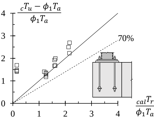
Figure 3-20 Concrete breakout failure strength evaluations of exposed column base with one side foundation beam
