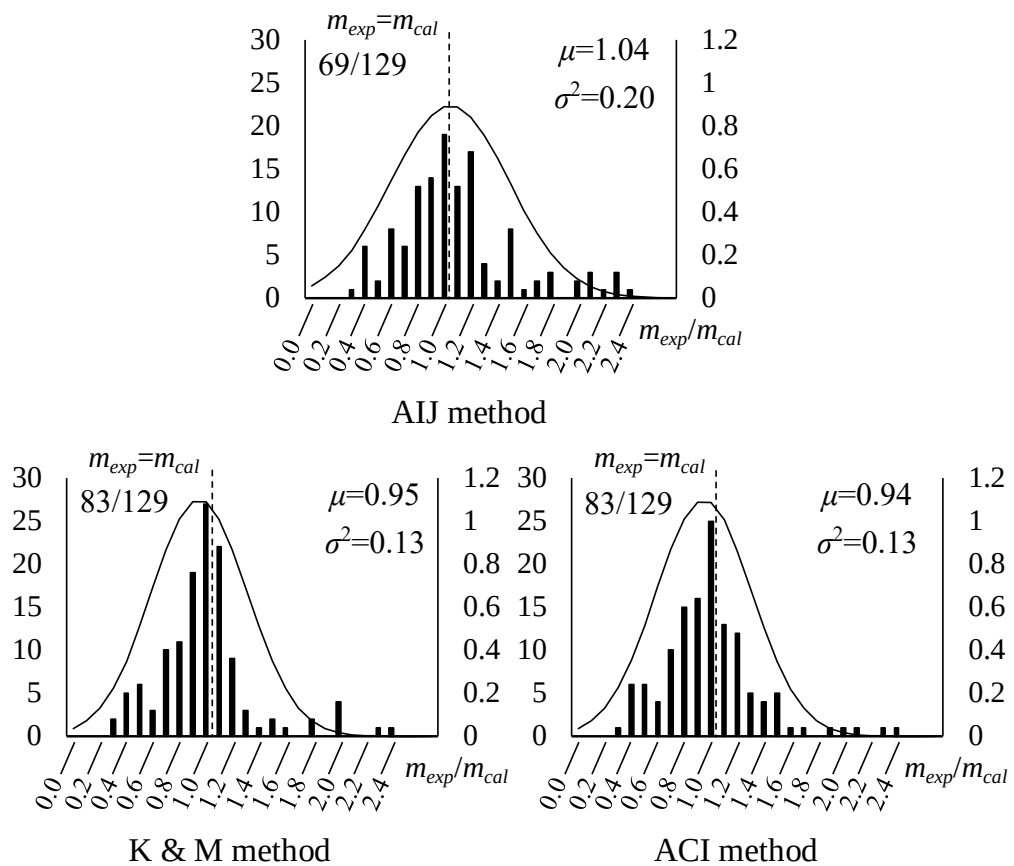
Figure 4-16 Statistical evaluation by existed calculation methods
