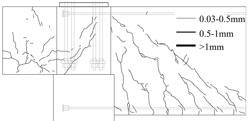
Hysteresis curve of Q - R and crack distribution when R = \pm 1/50
