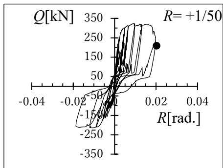
Hysteresis curve of Q - R and crack distribution when R = \pm 1/50
