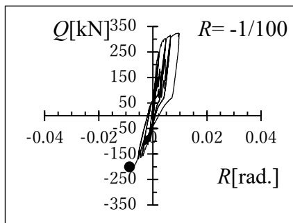
Hysteresis curve of Q - R and crack distribution when R = \pm 1/100
