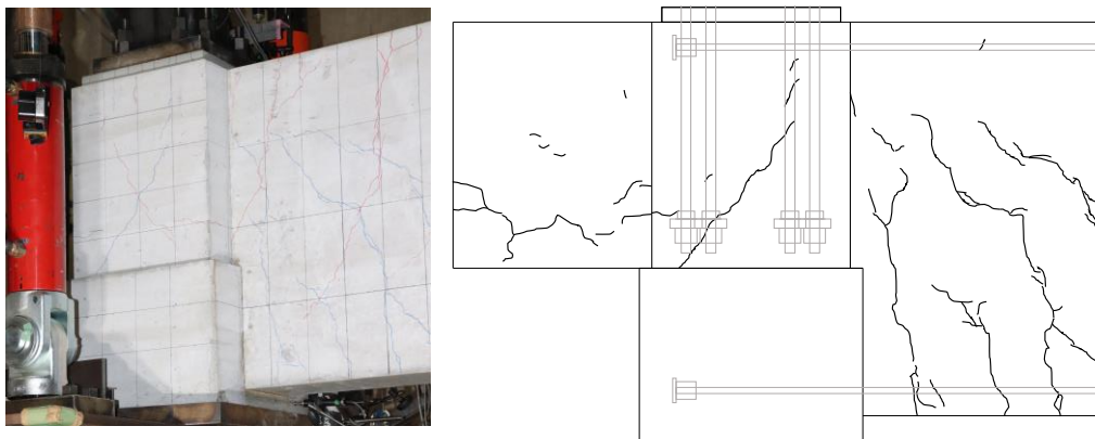
Figure 2-13 Concrete breakout failure cracks occurred in specimen B16-590-20d when R = +1/75
