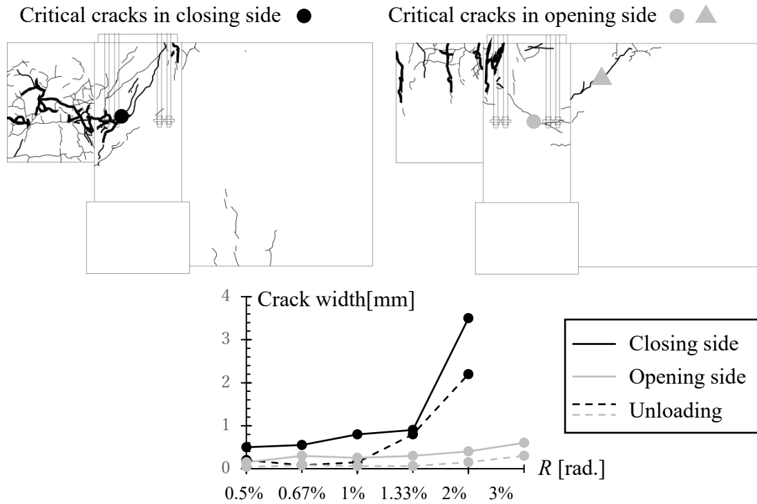
Increment of width of concrete breakout failure cracks
