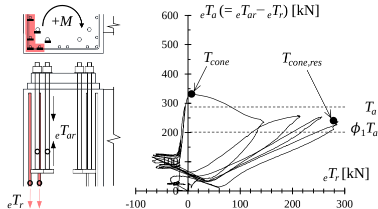
Figure 3-9 Strength relation of concrete and column rebar of specimen B16-590-20d
