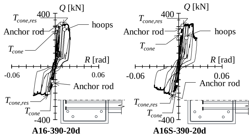
Figure 3-2 Hysteretic curve of A-series specimens
