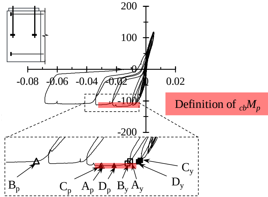
Figure 4-9 Definition of the full plastic strength cbM_p
