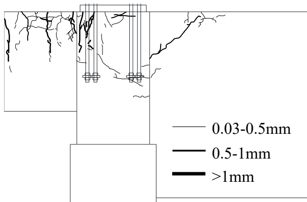
Hysteresis curve of Q - R and crack distribution when R = -1/33
