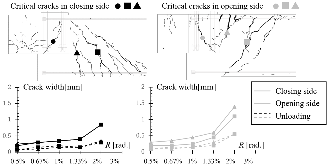
Increment of width of cracks on the foundation beam
