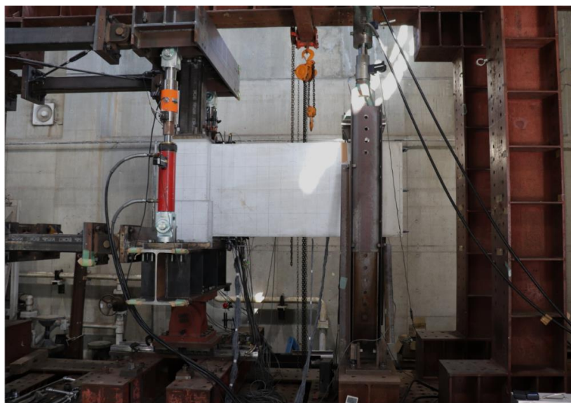
Photo 2-2 Experimental setup of B&C-series specimens
