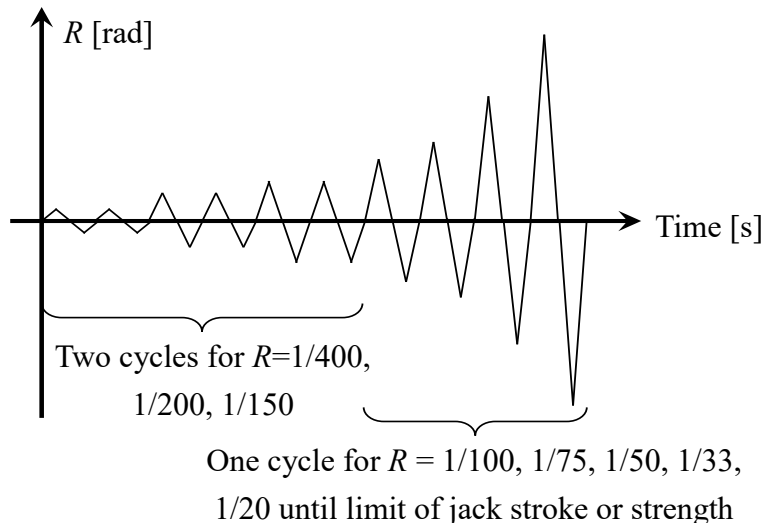
Figure 2-8 Loading protocol
