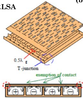
(c) Alternate-phase fed single mode waveguide
