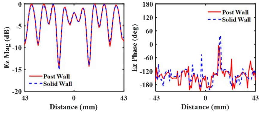
Figure 4.13: Field distribution along the center of the feeding waveguide
