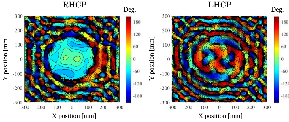
Figure 3.27: Measured aperture field distribution of the straight cross-slot feeding case at 5.9 GHz
