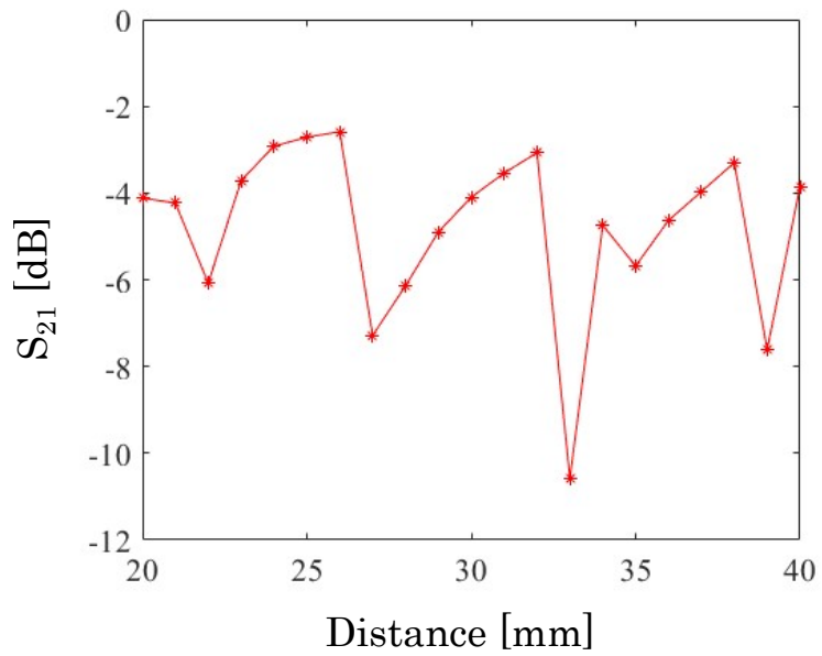
Figure 4.33: Transmission over the distances from 20 mm to 40 mm
