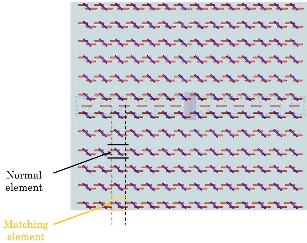
Figure 4.4: Radiating elements
