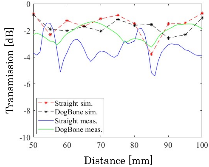
Figure 3.31: Plots of transmission over the distances from 50 mm to 100 mm
