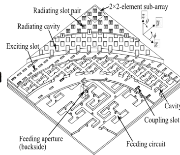
(e) Plate-laminated hollow-waveguide
