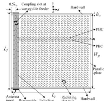
(b) Parallel-plate slot antenna
