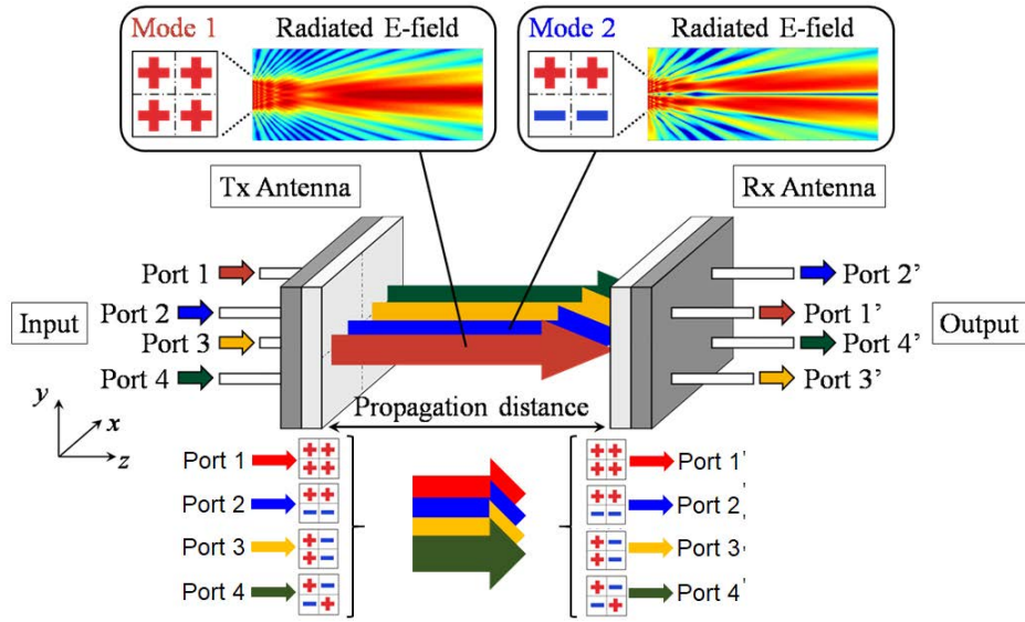
Figure 1.4: Rectangular orthogonal mode transmission system
