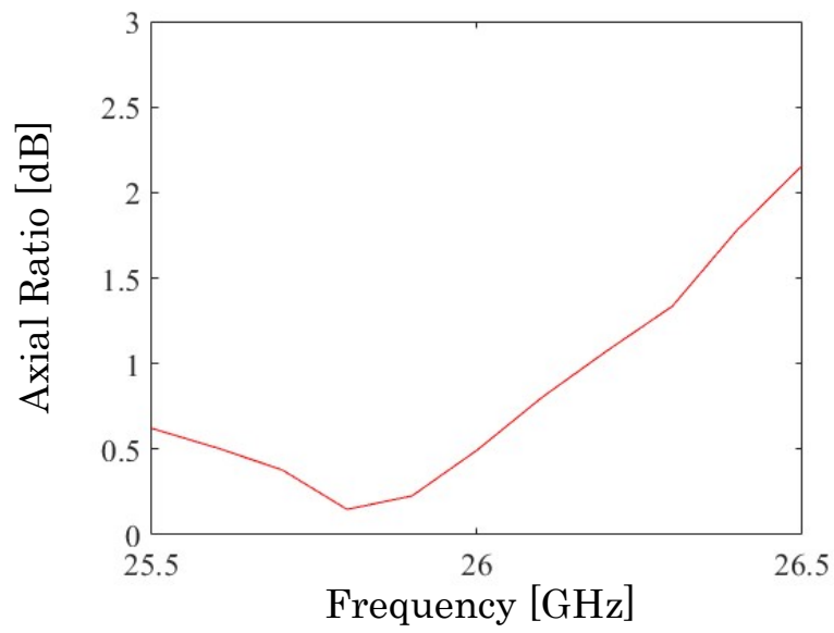
Figure 4.29: Plot of axial ratio of the full antenna model
