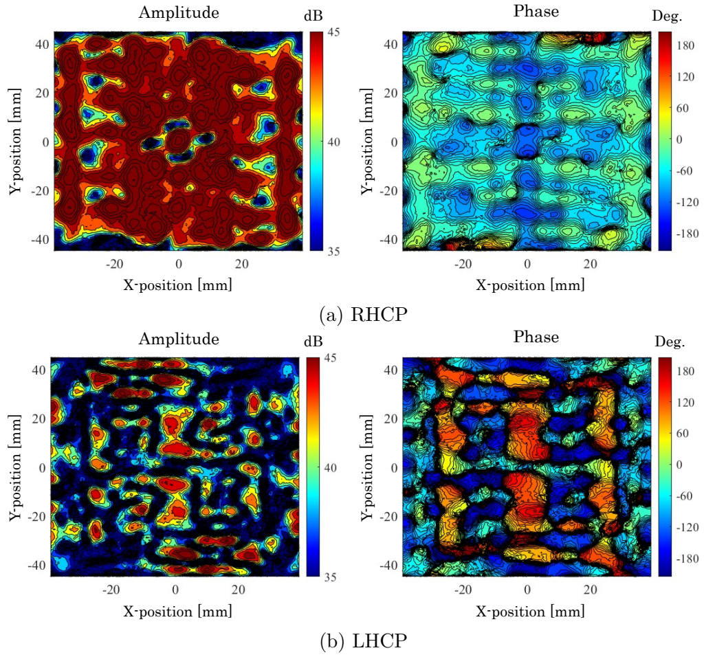
Figure 4.31: Aperture field distribution
