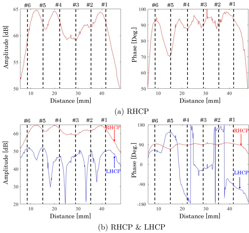
Figure 4.25: Field distribution along the center of the radiating elements
