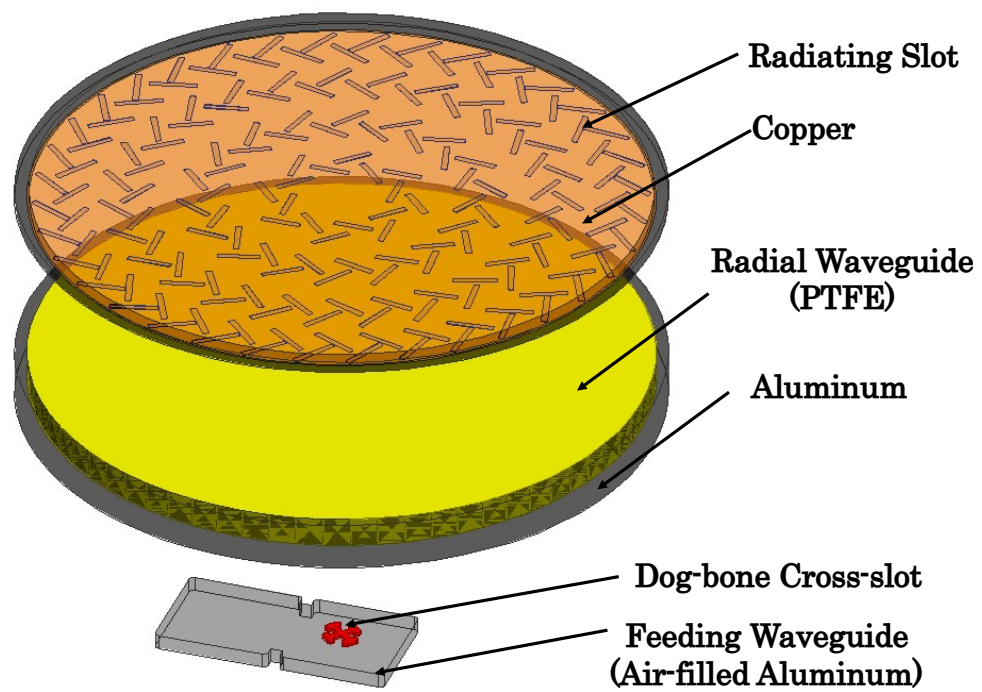
Figure 3.3: Antenna structure
