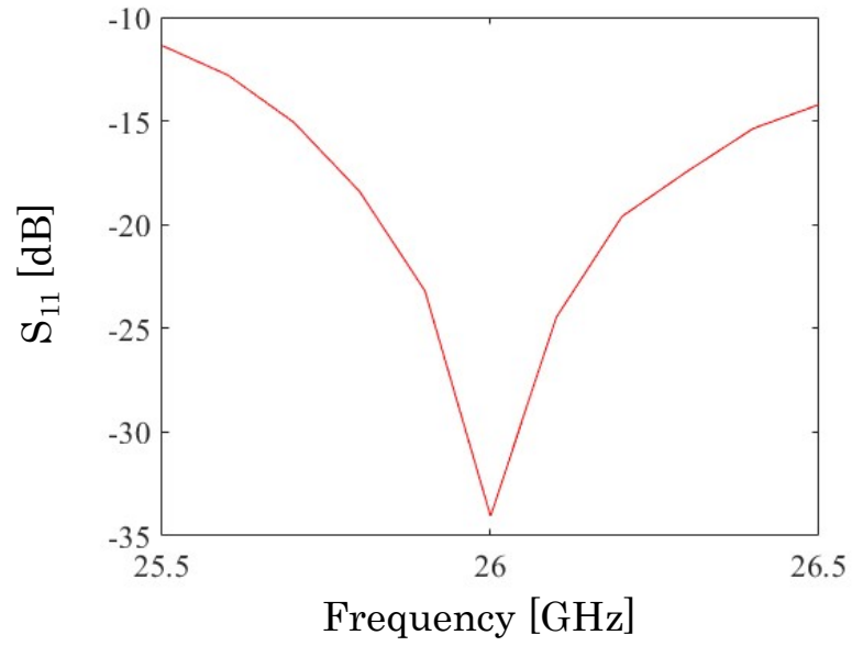
Figure 4.28: Plot of reflection of the full antenna model
