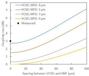
Fig. 3. Calculated/measured coupling loss from VCSEL to SMF.
