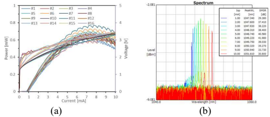
Fig. 2: (a) IL characteristics of all 16 devices in an array and (b) lasing spectra for a typical device with different currents.
