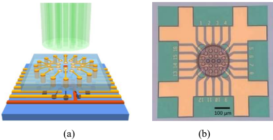
Fig. 1: (a) The schematic view of a VCSEL array coupling to a multi-core fiber; (b): top-view of a fabricated VCSELs array.
