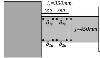
Fig. 5 Evaluation of rotation angle _{test}\theta_B from experiment
