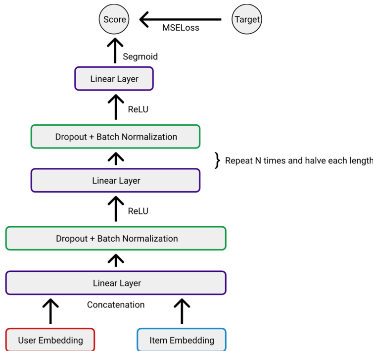
Figure 1. Neural network structure of NCF part
