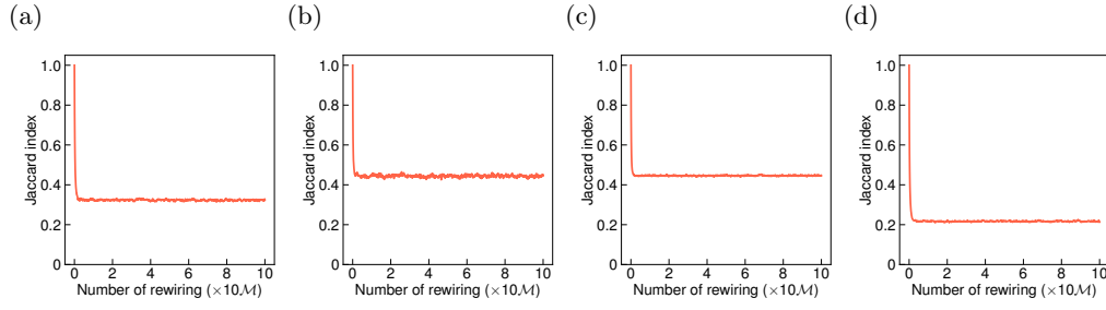
Figure 4.10: The Jaccard index between a set of edges of the empirical hypergraph and that of the hypergraph generated under the randomizing rewiring. We set (d_v, d_e) = (2, 1) . (a) Drug, (b) Enron, (c) primary-school, and (d) high-school. The Jaccard index between the sets of edges is given by |\mathcal{E} \cap \tilde{\mathcal{E}}|/|\mathcal{E} \cup \tilde{\mathcal{E}}| , where \mathcal{E} and \tilde{\mathcal{E}} are the set of edges in the original and synthetic hypergraphs, respectively. In calculating the Jaccard index, we removed multiplicity of edges in \tilde{\mathcal{E}} .
