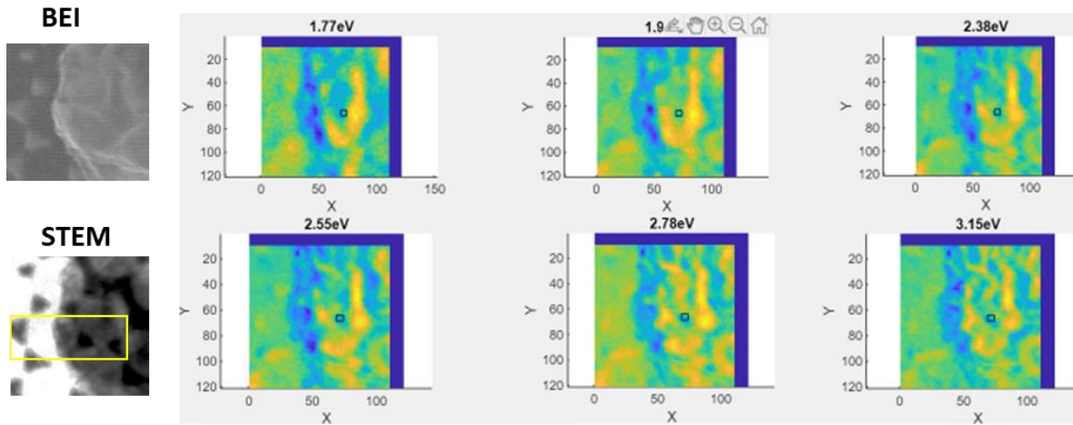
Figure 6.1 Subtraction of CL map at the beam current of 4.5 nA to 0.25 nA with normalized CL intensity.
