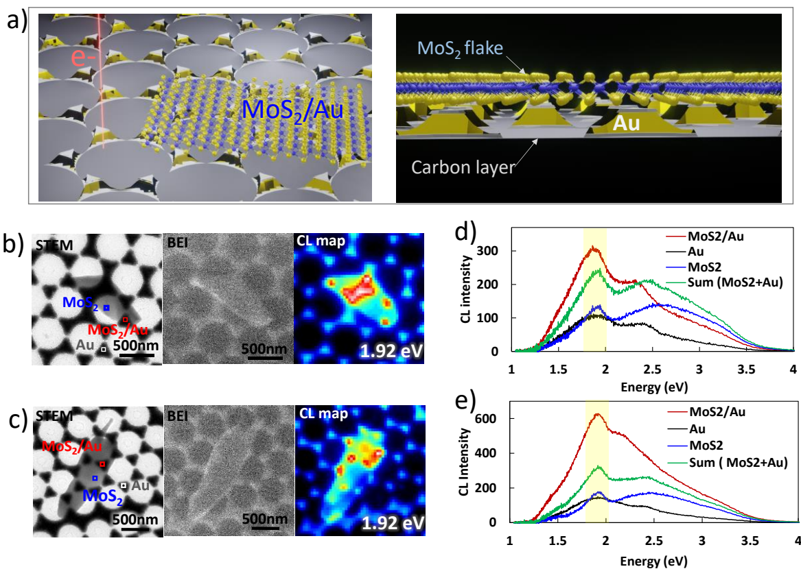
Figure 4.7. Structure and CL properties of MoS 2 -Au pyramids hybrid structure. a) Schematics of MoS 2 -Au pyramids hybrid structure, where MoS 2 flakes were drop-casted above the Au nanopillar arrays which supported by a thin carbon layer. b) and c) STEM bright-field images, BE images and corresponding CL maps of two positions of MoS 2 -Au pyramids hybrid structure. d) and e) CL spectra extracted from CL maps in b and c for MoS 2 (in blue line), Au pyramids (in black line), MoS 2 - Au pyramids, and sum of MoS 2 plus Au pyramids (in green line). CL signals were collected normally from all radiation angles without polarization and masks.
