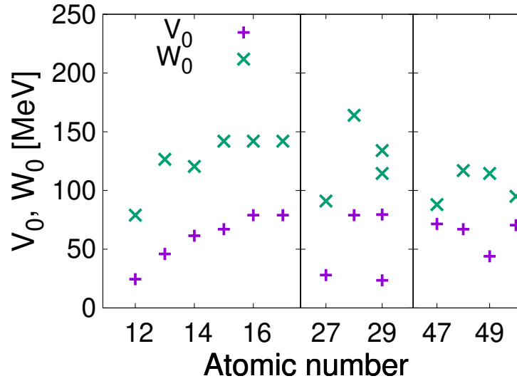
Fig.7.4 Atomic dependence of the potential parameters for Potential 1. The plus (+) and cross (×) signs denote the parameters for the real and imaginary parts, respectively.
