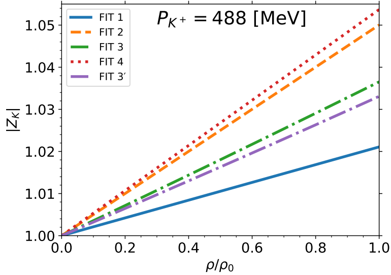
Fig.6.14 The density dependence of the absolute value of the wavefunction renormalization factor Z_K at the P_{K^+} = 488 \text{ MeV}/c .
