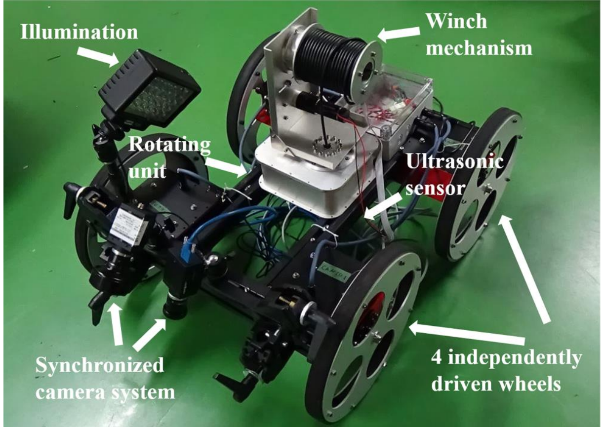
Figure 2.2 The hardware prototype of test platform RhinoUS-II.
