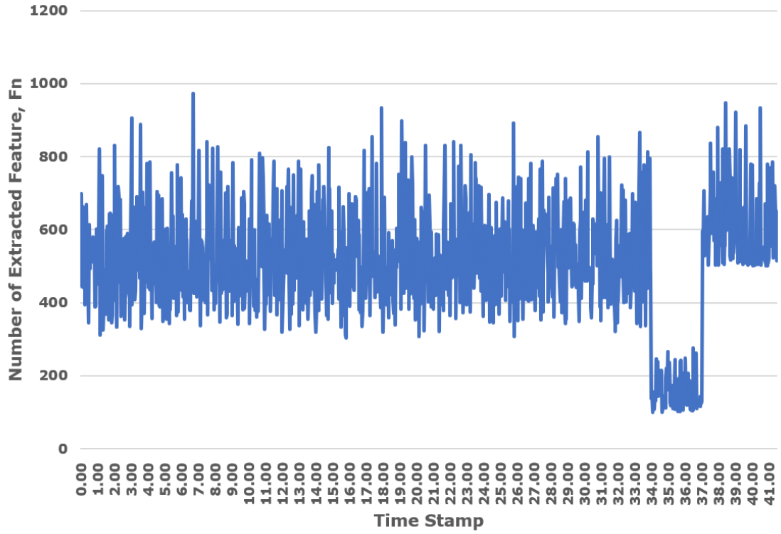
Figure 3.16 The number of extracted feature points F_n according to the time stamp in the test run image sequence.
