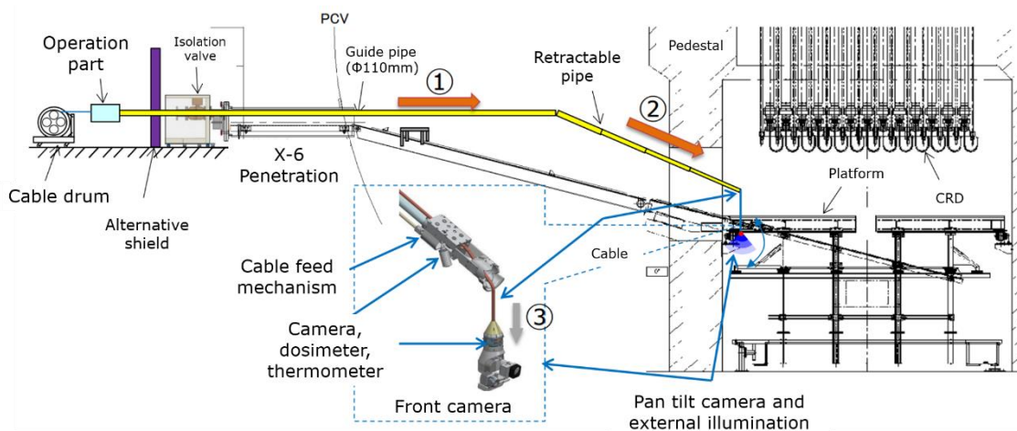
Figure 1.7 The investigation setup of investigation A2’.
