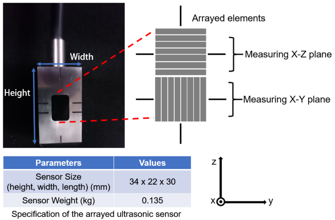
Figure 2.11 The prototype 2D phased array ultrasonic sensor.
