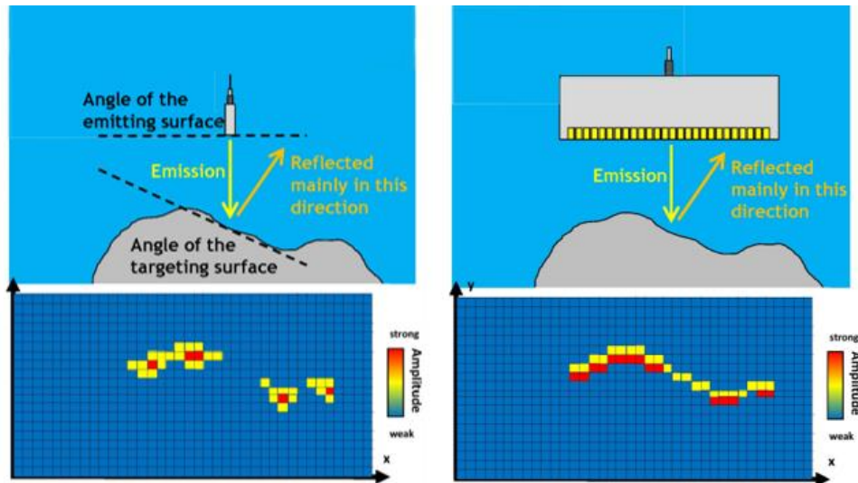
Figure 0.3 Schematics of the aperture synthesis method. Left: Measurement with conventional ultrasonic sensor; Right: Measurement with aperture synthesis method and array sensor. [35]
