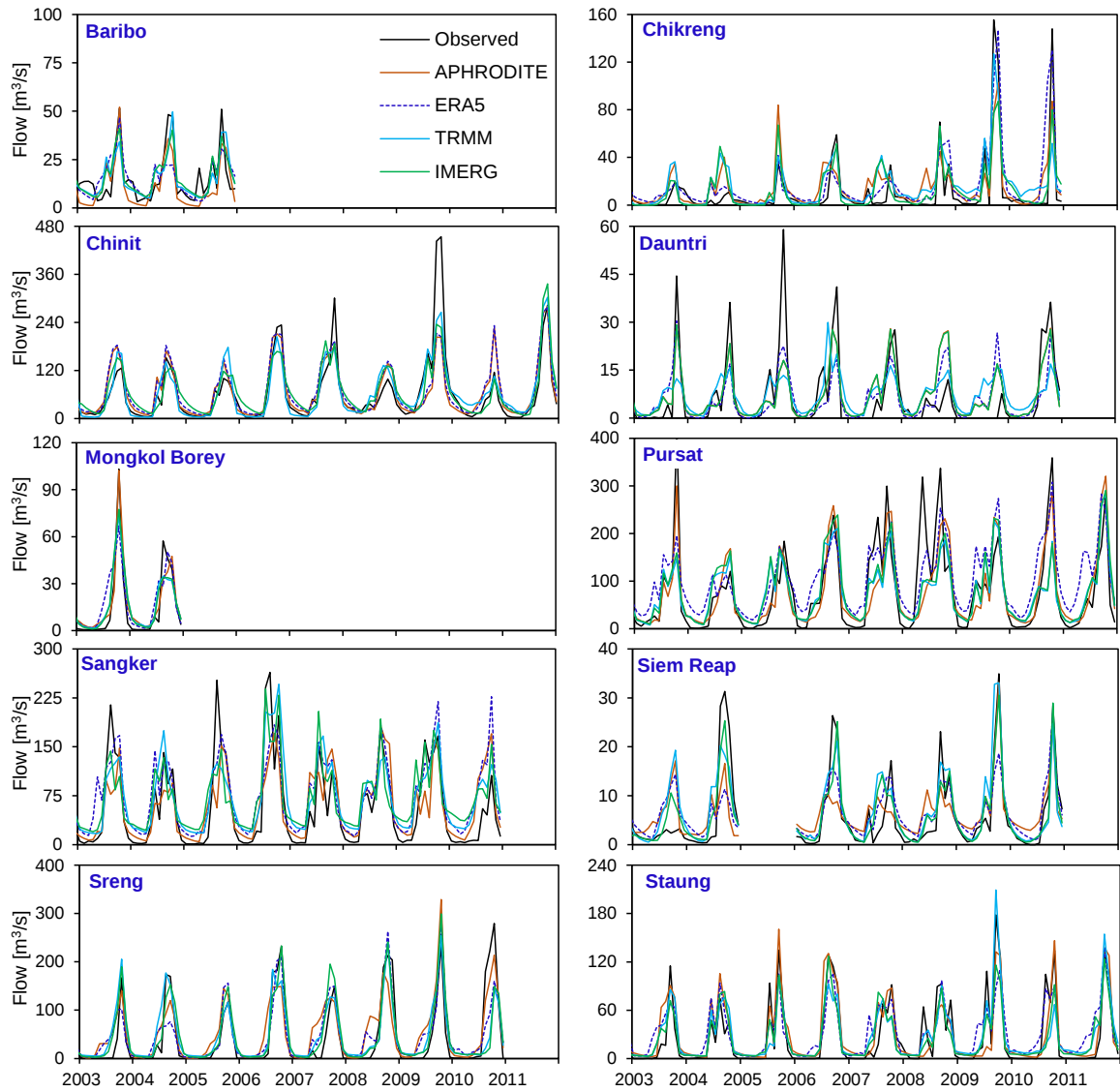
Figure A7. Same as Figure A6 but for the validation period. Due to discontinued monitoring stations in Mongkol Borey and Baribo tributary basins, the flow simulations were validated from 2003 to 2004 and 2005, respectively. The flow data of the Siem Reap tributary basin was missing in the year 2005, thus; the model was validated from 2003 to 2004 and 2006 to 2010.
