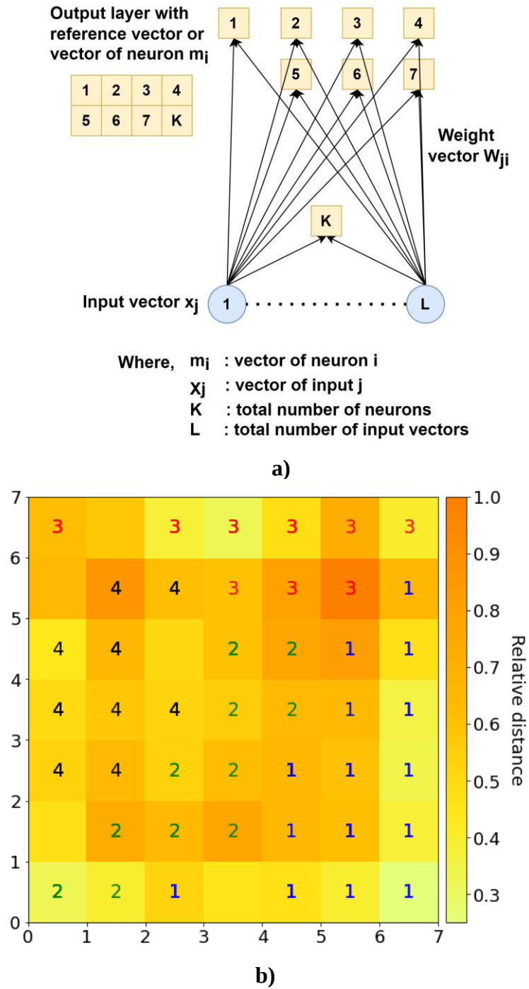
Figure 3.2. a) Schematic diagram of the self-organizing map. b) Unified distance matrix (U-matrix). In b), the number shown on the map denotes clusters. Colors denote the relative distance between the grids numbered on each axis.
