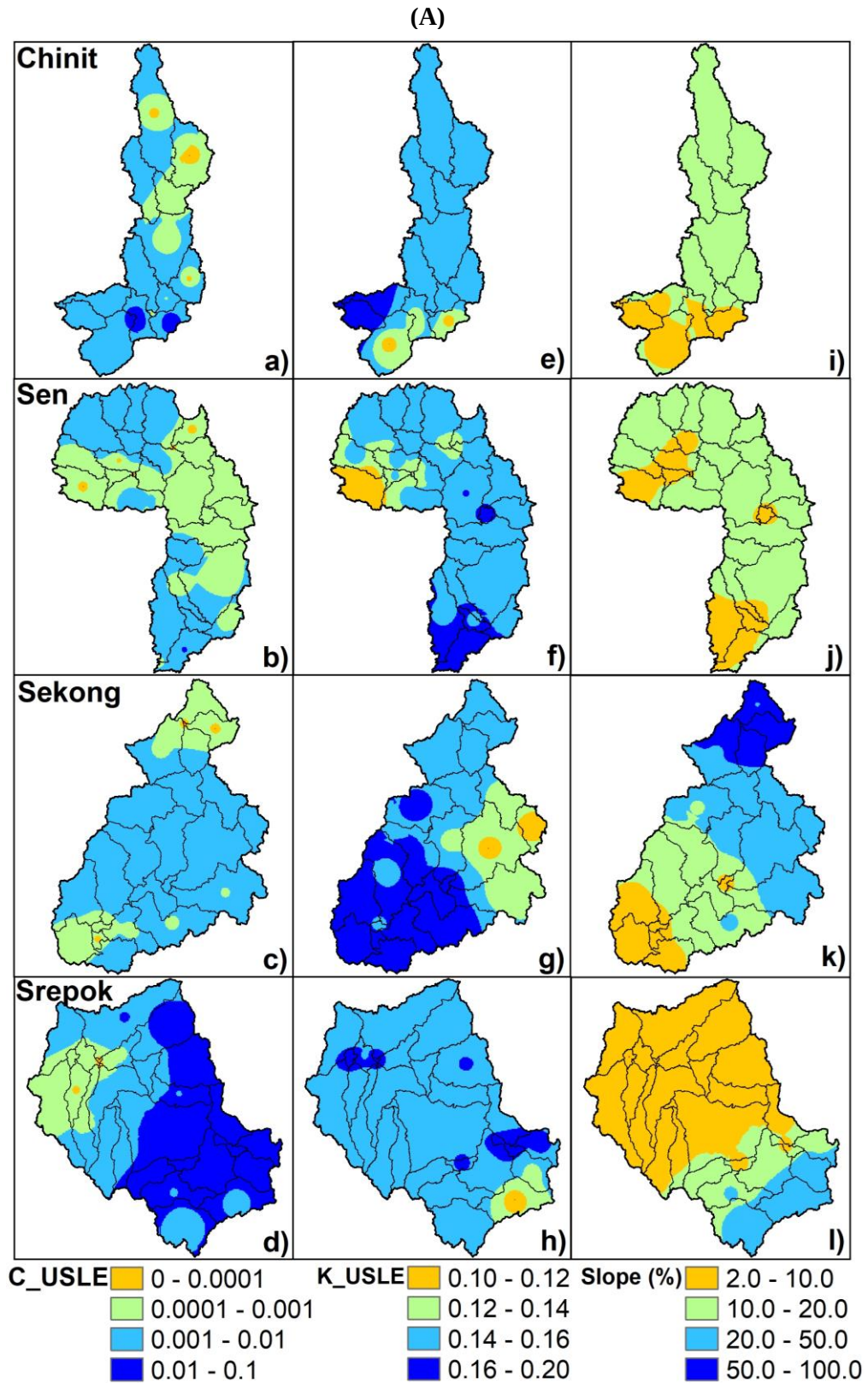
Figure 3.4. (A) Area-weighted values of C_{USLE} (a-d), K_{USLE} (e-h) and slope percentage (i-l) for the physical similarity regionalization method. (B) Coefficient of variation of rainfall (m-p), coefficient of variation of sediment load (q-t) and correlation coefficient between rainfall and sediment load (u-x) for the sediment-response similarity regionalization method.
