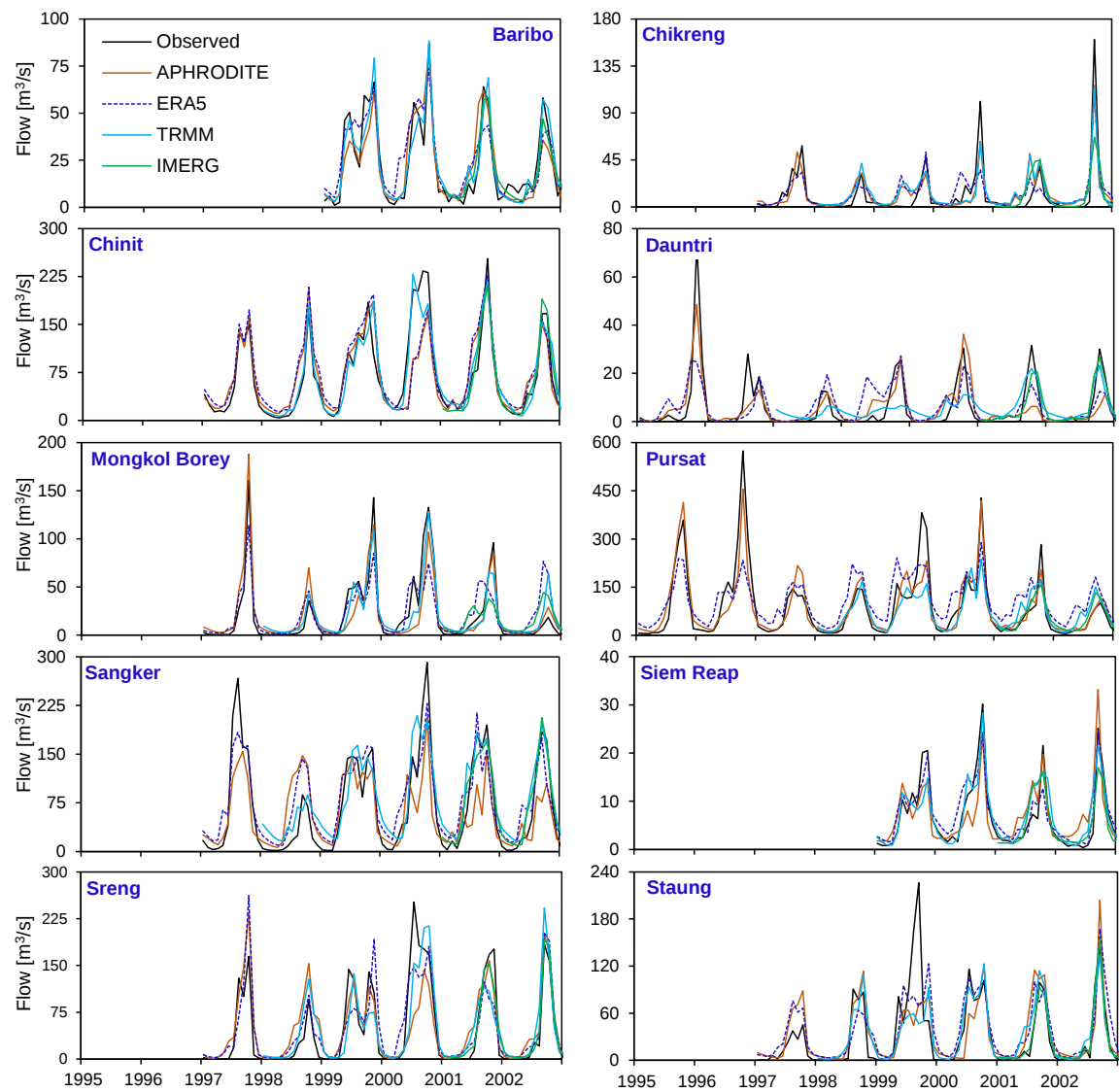
Figure A6. Monthly observed and simulated flow of each tributary basin in the calibration period. The beginning of the flow simulation depended on the flow data availability of each tributary basin.
