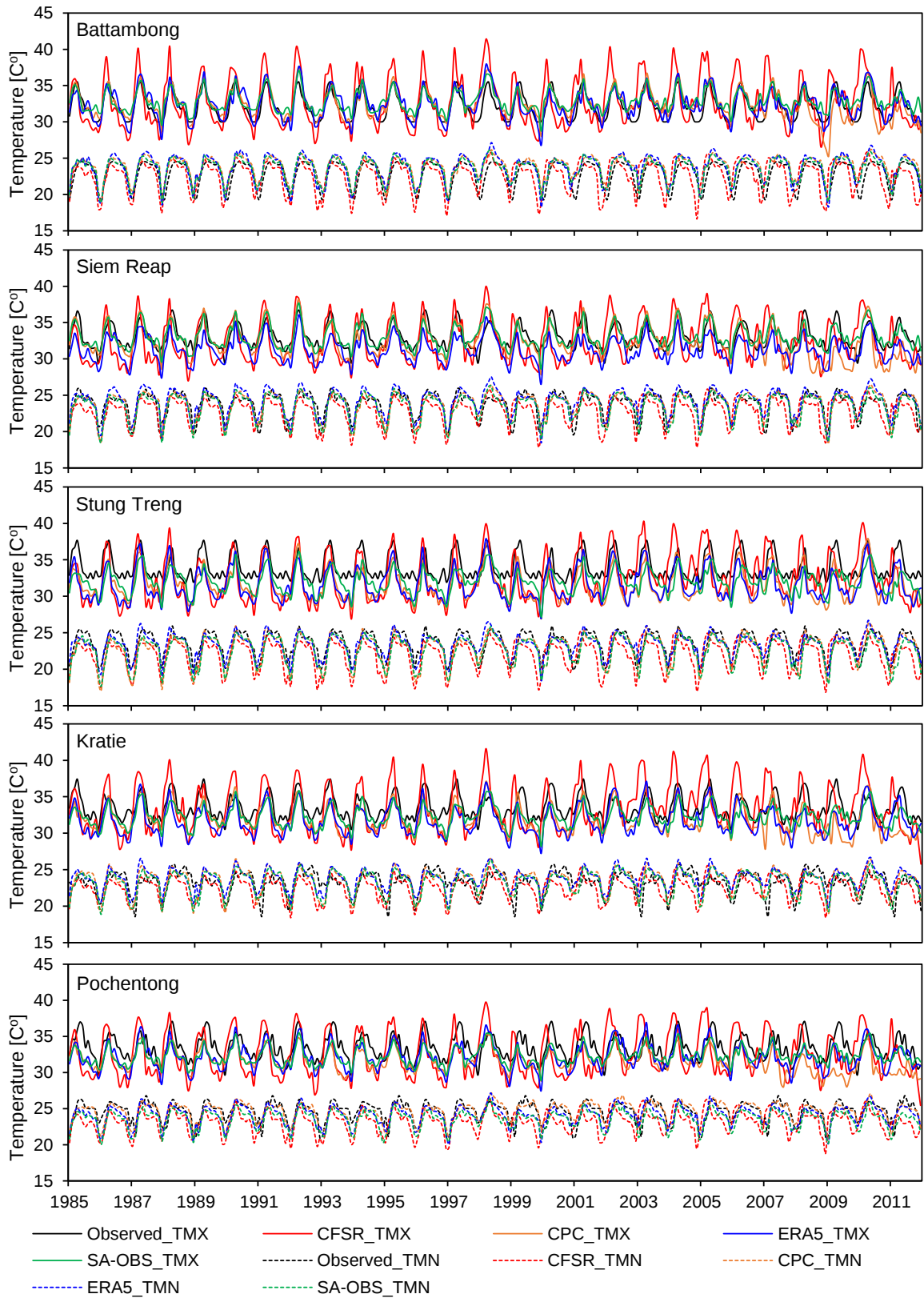
Figure A5. Comparison of monthly mean daily maximum (TMX) and daily minimum (TMN) temperatures of individual stations from 1985 – 2011. The different colors of solid- and dash-lines denote the maximum and minimum temperature, respectively, of different datasets.
