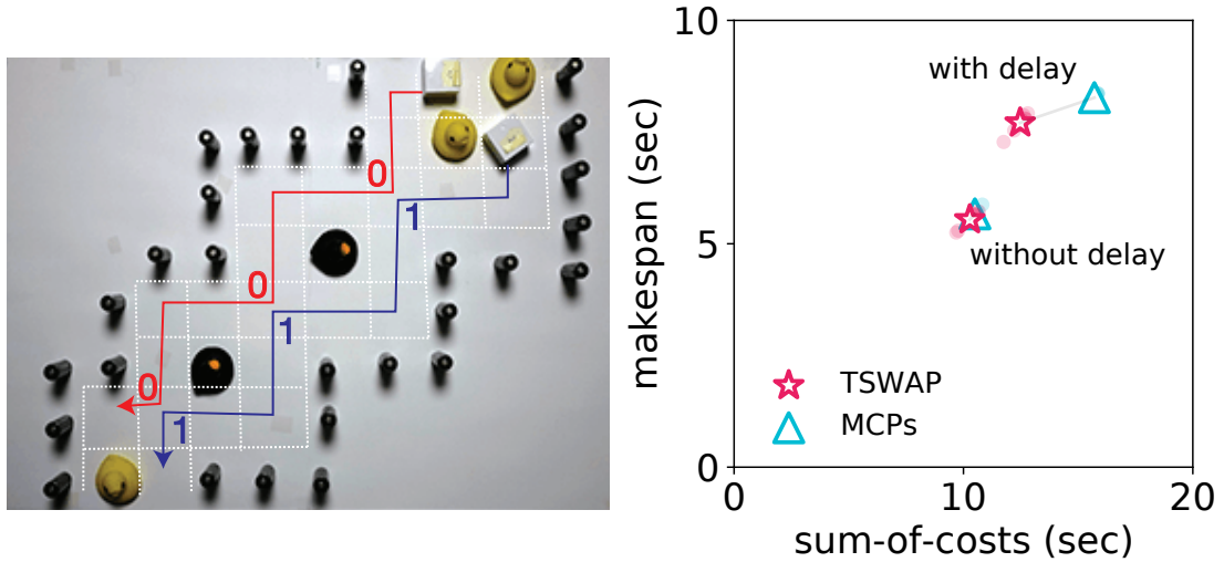
Figure 8.2: Demonstrations of delay tolerance. left: The initial configuration and the offline plan, accompanied by temporal orders, used in MCPs are illustrated. Targets are shown by the tips of arrows. The red one's speed was made half in one scenario (with delay). right: Average sum-of-costs. Scatter plots of ten repetitions are plotted by transparent points.
