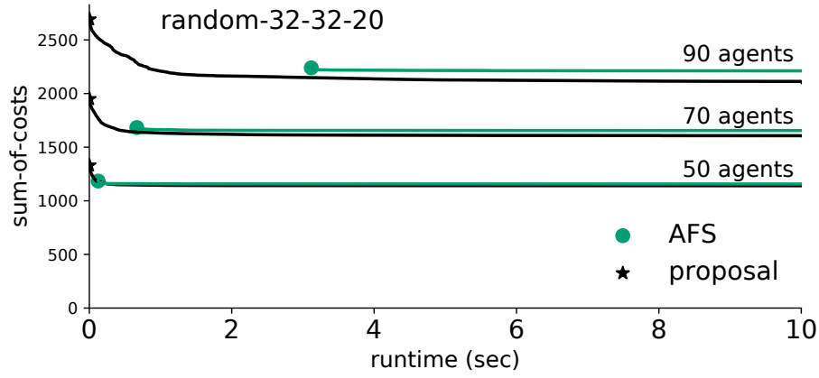
Figure 7.9: Results vs. another anytime MAPF solver. We omit scores after 10 s because they are almost flat. The improvements of AFS were subtle and hard to recognize. ©2021 IEEE.
