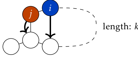
Figure 7.1: Example of local minimum. Goals are depicted by arrows.
