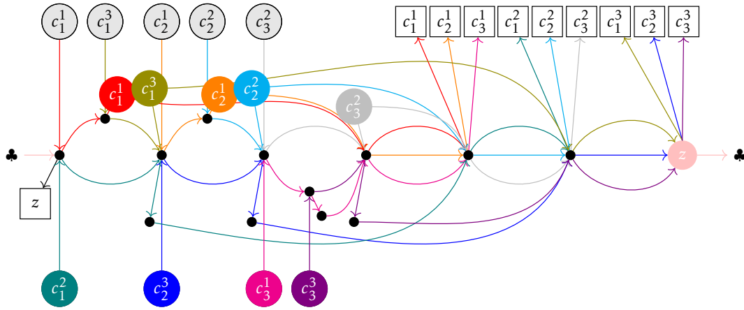
Step 1: Move assigned agents to vacation vertices
