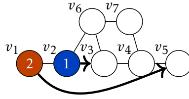
Figure 7.2: Example of local repair around goals.
