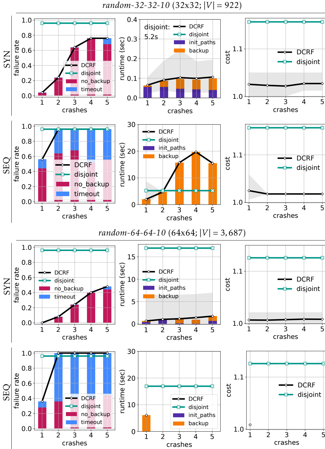
Figure 10.13: Results with a fixed number of agents ( |A| = 15 ).
