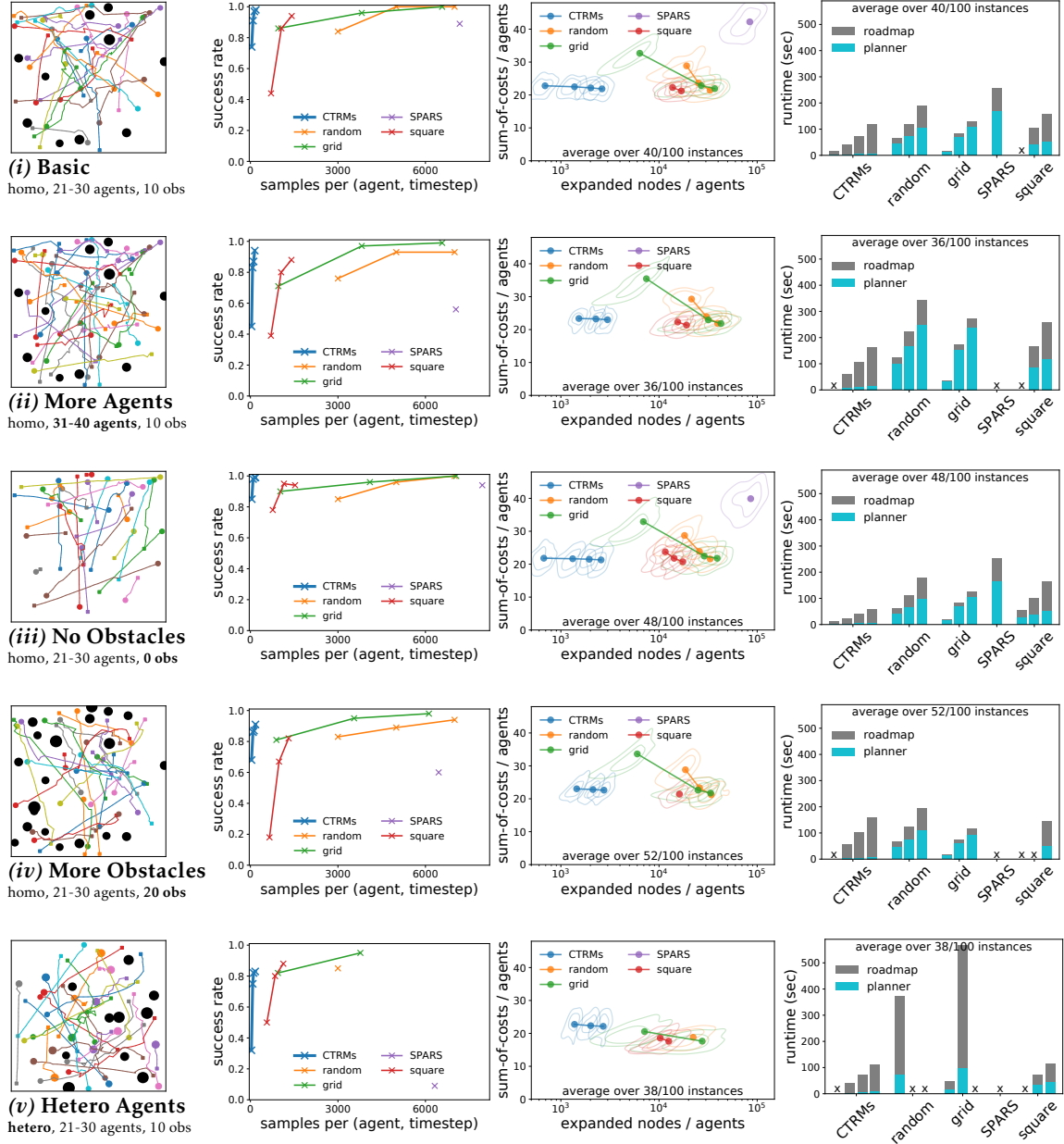
Figure 11.5: Summary of results. The rows correspond to respective scenarios. For each method, plots to the right correspond to the denser roadmaps (e.g., CTRM: n_{\text{traj}} = 25 \rightarrow n_{\text{traj}} = 100 , grid: 32 \times 32 \rightarrow 84 \times 84 ). First column: Solution examples planned by PP on CTRM ( n_{\text{traj}} = 25 ). Second column: Success rate vs. the number of samples per agent and per timestep in the constructed roadmaps. Third column: Sum-of-costs vs. the number of expanded search nodes in the planning phase. Each value is normalized by dividing by the number of agents. Fourth column: Overall runtime, consisting of the planning and the roadmap construction phases. For the results in the third and fourth rows, in order to obtain meaningful insights, several methods with success rates below 70% were excluded; the scores have calculated the average of the metrics for problem instances where all the remaining methods were successful in planning. Some baselines with specific parameter settings are also omitted due to extremely long computation times (over 15 min per problem instance) from the evaluation of the Hetero Agent scenario. All these omitted methods and settings are marked with “x” in the fourth row.
