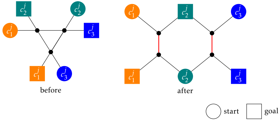
Figure 9.16: Equivalent gadget of the clause constrainer for a clause C^j .
