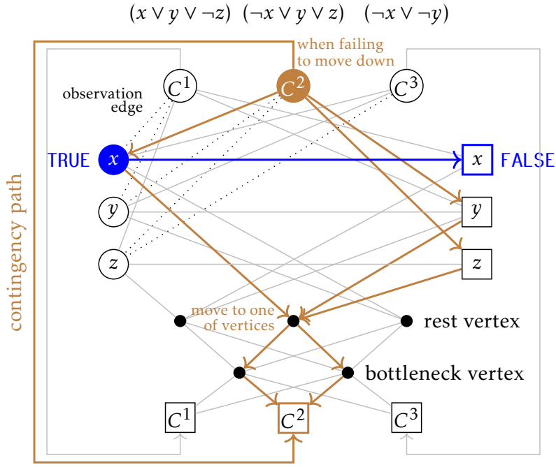
Figure 10.8: MAPPCF instance and solution reduced from SAT. The corresponding formula is (x \vee y \vee \neg z) \wedge (\neg x \vee y \vee z) \vee (\neg x \vee \neg y) . Dotted lines are edges that are not used in the plans.
