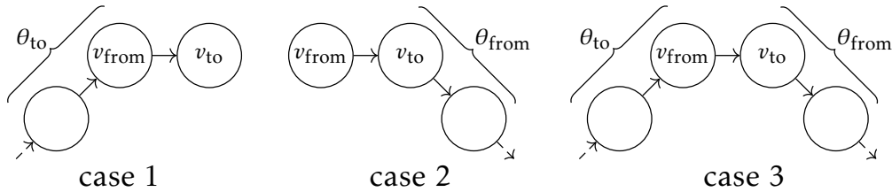
Figure 9.11: Three cases of creating new fragments by extending existing fragments.
