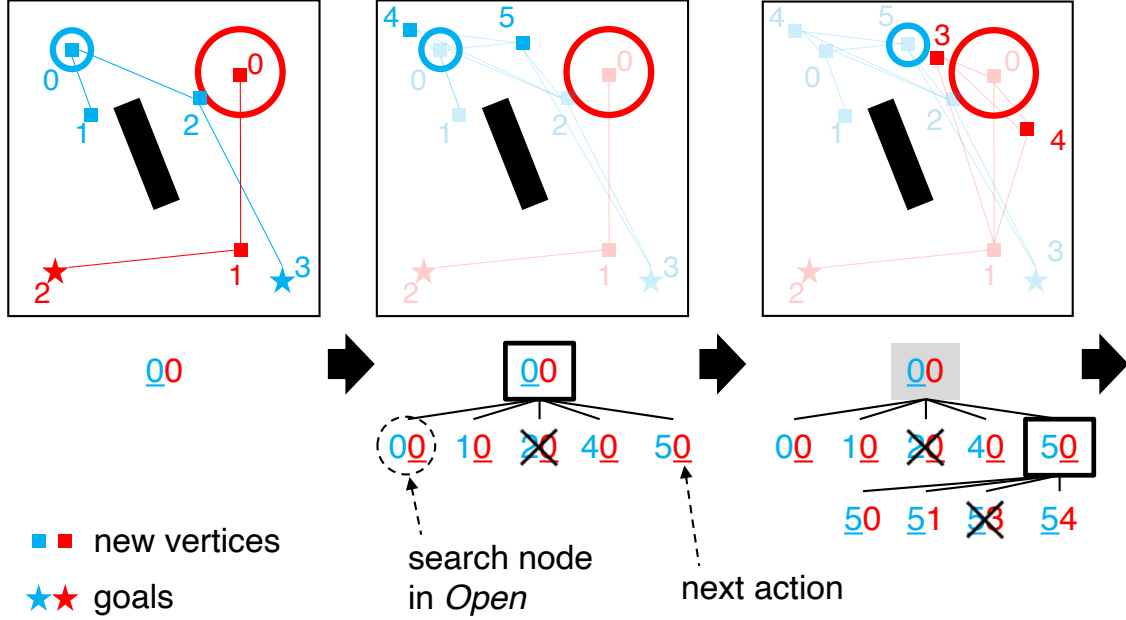
Figure 12.1: Illustration of SSSP. The algorithm progresses from left to right. top : Robot-wise roadmaps and search situations. Two robots are shown by colored circles and an obstacle by a black rectangle. bottom : Search trees. A node ' xy ' corresponds to a situation where the blue and red robots are respectively at vertices ' x ' and ' y ', and the blue robot will take the next action. left : Initial roadmaps. The search starts from the node ' 00 .' middle : Vertex expansion and search node expansion for the blue robot. The node ' 20 ' is not expanded due to inter-robot collision. right : The red robot's turn. The search continues until all robots reach their goals.
