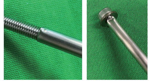
Fig. 8: Buckling of the pipe ends where wall-thickness is 0.2 mm
