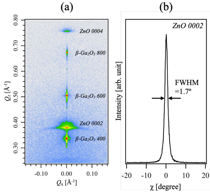
Figure 5.12 (a) RSMs of ZnO thin films grown on \beta\text{-Ga}_2\text{O}_3 single crystal buffered COP substrate and (b) rocking curves of ZnO 0002 diffraction.
