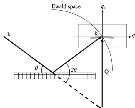
Figure 2.7 Schematic diagram of reciprocal space mapping using a two-dimensional detector.
