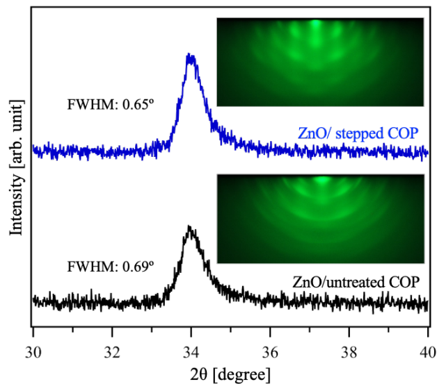
Figure 3.4 XRD 2\theta/\theta profiles and RHEED patterns (inset) of ZnO thin films grown on untreated and stepped COP substrates.
