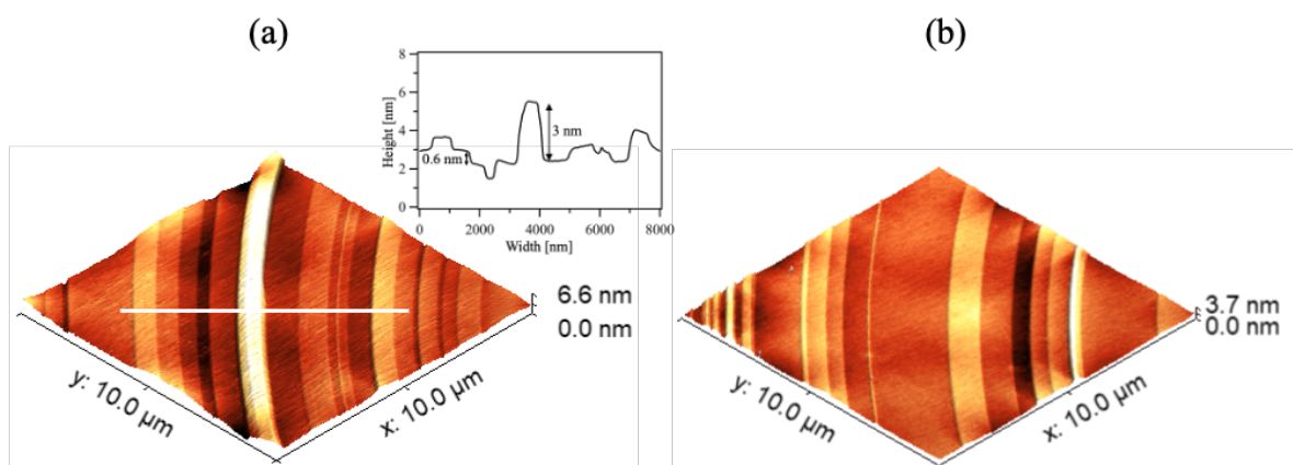
Figure 5.9 AFM images of the surface of (a) cleaved \beta -Ga 2 O 3 (100) single crystal buffer layer on COP substrate and cross-sectional profile along atomic steps and terrace structures, and (b) ZnO thin film grown on COP substrate with \beta -Ga 2 O 3 (100) single crystal buffer layer.
