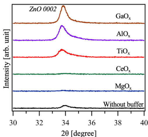
Figure 5.1 XRD 2\theta/\theta profiles of ZnO thin film grown on COP substrates with or without oxide buffers.
