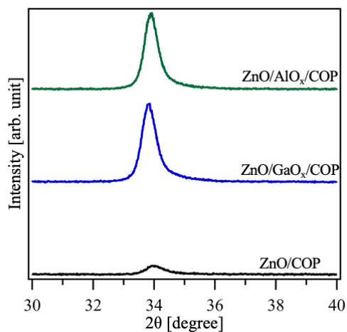
Figure 5.4 XRD 2\theta/\theta profiles of ZnO thin films grown on COP substrates with AlO x or GaO x buffer layers of 100 nm and without buffer layers.
