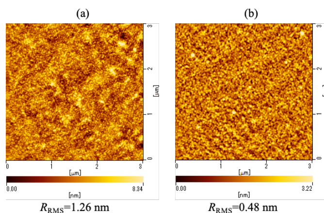
Figure 6.3 AFM images of AZO thin films ( t \sim 200 nm) grown on (a) untreated and (b) stepped and \text{AlO}_x buffered COP substrates.
