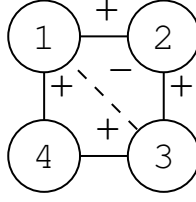
Figure 5.1: An aggregated sparsity pattern graph with edge signs. The solid and dashed lines show that the corresponding \sigma_{ij} are +1 and -1 , respectively. Both lines indicate the existence of nonzero elements in some Q^p .
