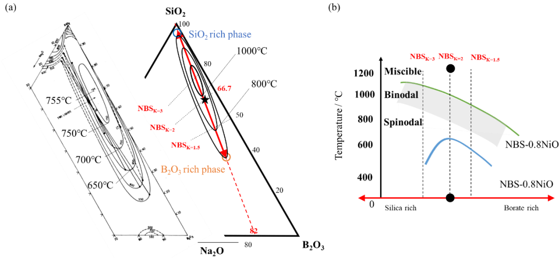
Figure 4.9 (a)(b) Approximate phase separation domain marked in ternary diagram of Na 2 O-B 2 O 3 -SiO 2 after doping NiO. The main composition is marked with star. The reference diagram of Na 2 O-B 2 O 3 -SiO 2 without NiO is from [104].
