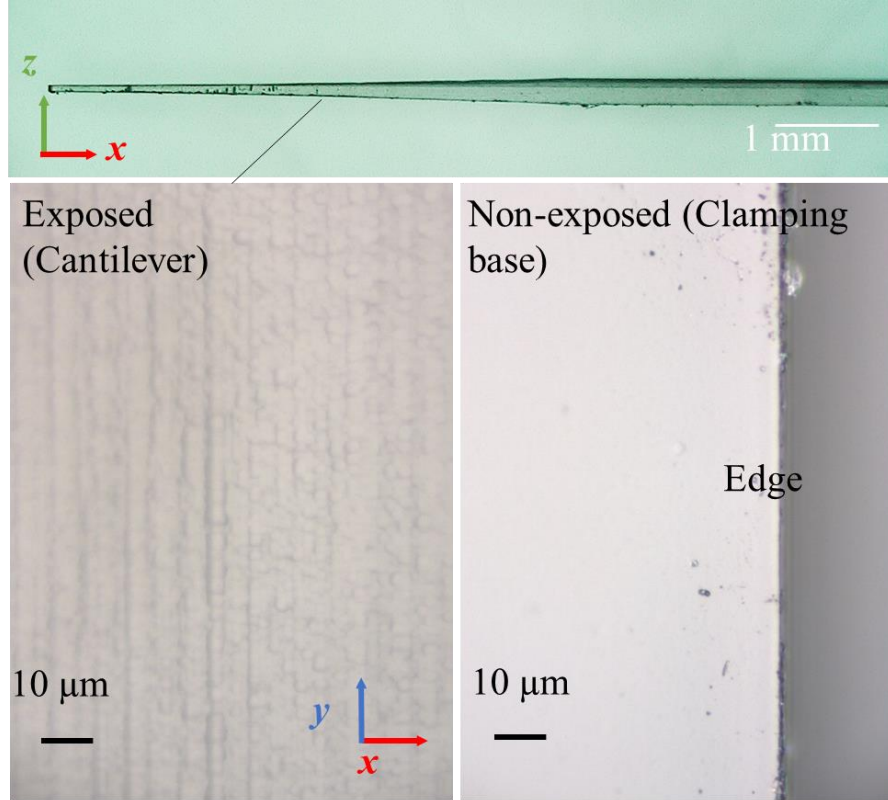
Figure 6.3 Appearance of the fabricated cantilever with tapering. Top: Side view of fabricated cantilever ( L_{\text{Taper}}=5 mm), Bottom: Microscopic photographs of laser exposed surface (left) and non-exposed one (right) of cantilever.
