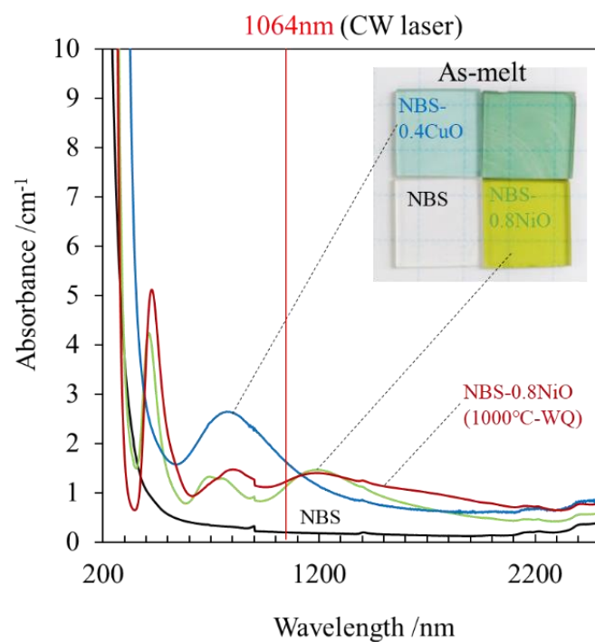
Figure 5.4 UV-vis absorption spectra of the glasses with target composition.
