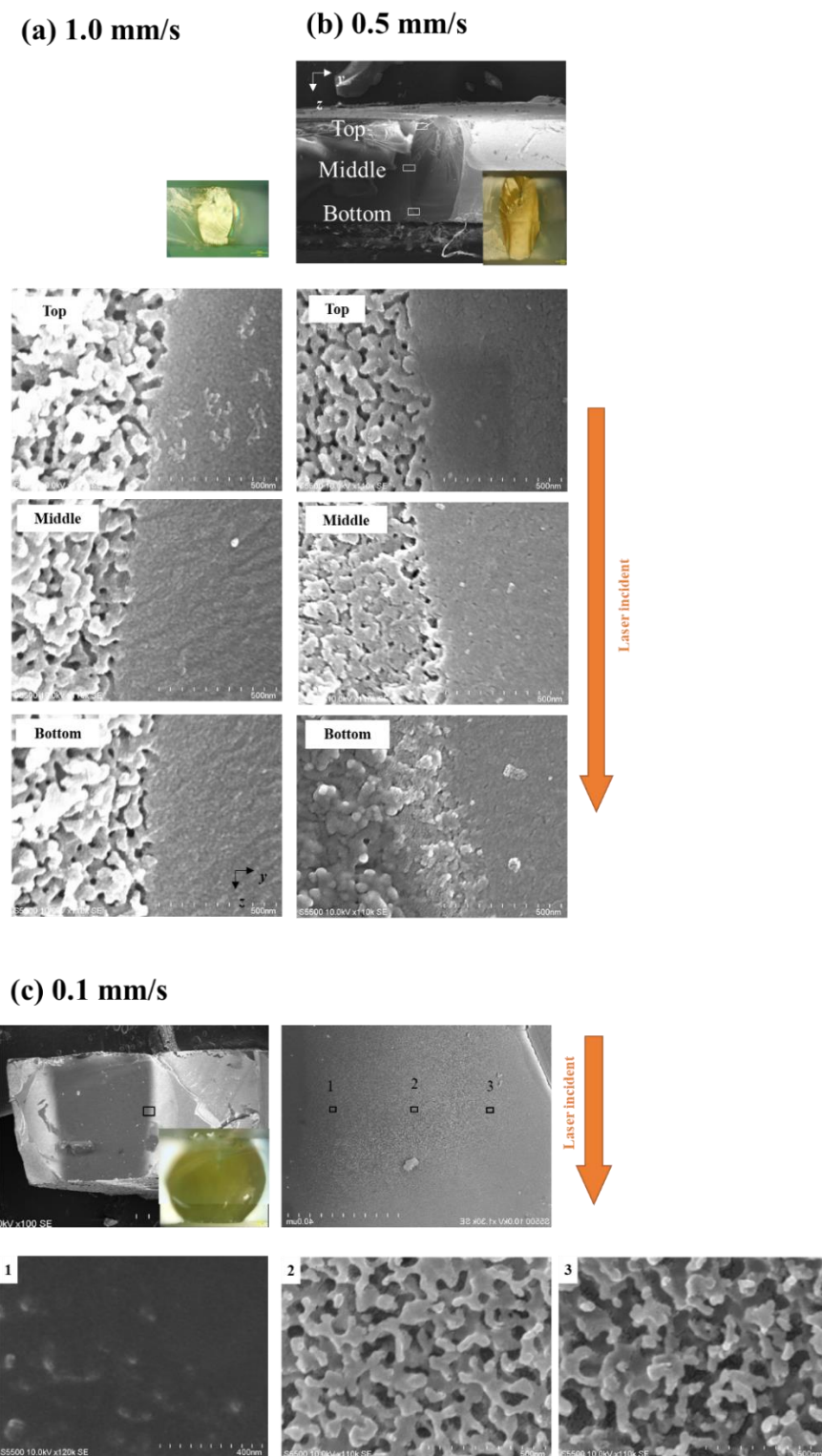
Figure 2.11 The porous/ non-porous boundary at top, middle, bottom part along laser incident direction. The phase separated glass plates were irradiated with 4.3 W with different scanning speed. (a) 1.0 mm/s, (b) 0.5mm/s, and (c) 0.1 mm/s.
