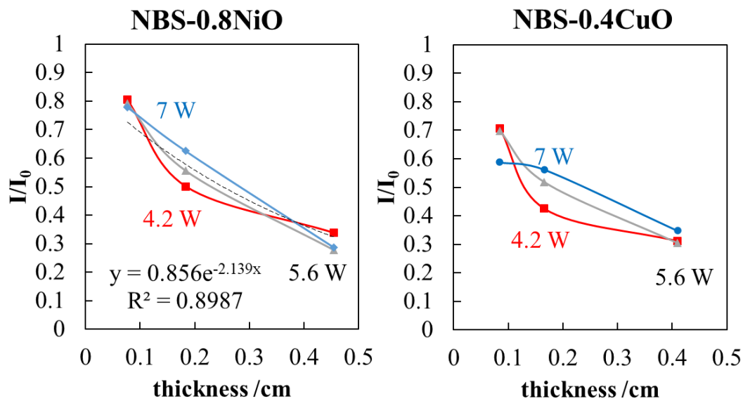
Figure 5.5 Laser ( \lambda=1064 nm) intensity ratio (transmittance) in NBS-0.8NiO and NBS-0.4CuO glass substrate during heating at 100^{\circ}\text{C} with different thickness.
