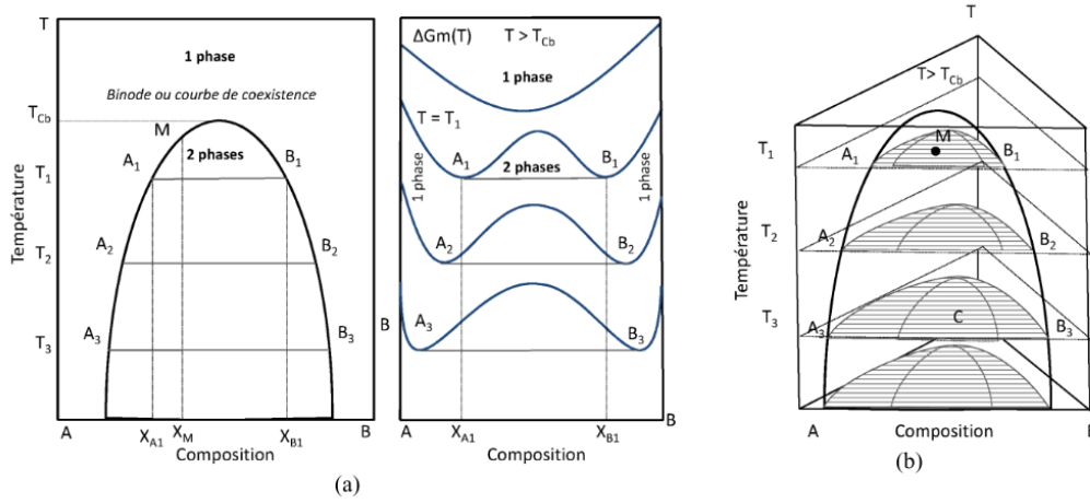
Figure 1.1 Composition and temperature dependence of phase separation in binary system. When the glass with certain composition is exposed under temperature located inside the illustrated dome in (a), glass shows immiscibility to give two different compositions A and B spotted on the dome line. In case of ternary system, it can approximated as binary phase separation by fixing one component which has small effect on phase separation behavior, indicated as “C” in (b) [33]
