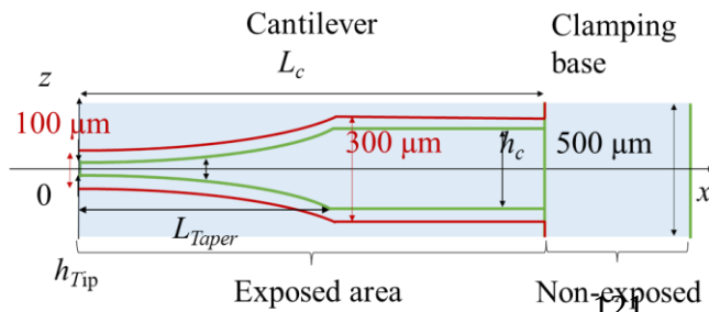
Figure 6.2 Schematic illustration of laser scanning process to pick out the tapered cantilever of the silica glass substrate.
