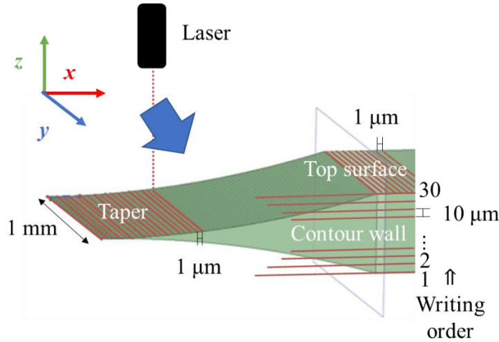
Figure 6.1 Dimension of cantilever and position inside silica glass substrate. Laser irradiated surface in red line and actual surface in green line.
