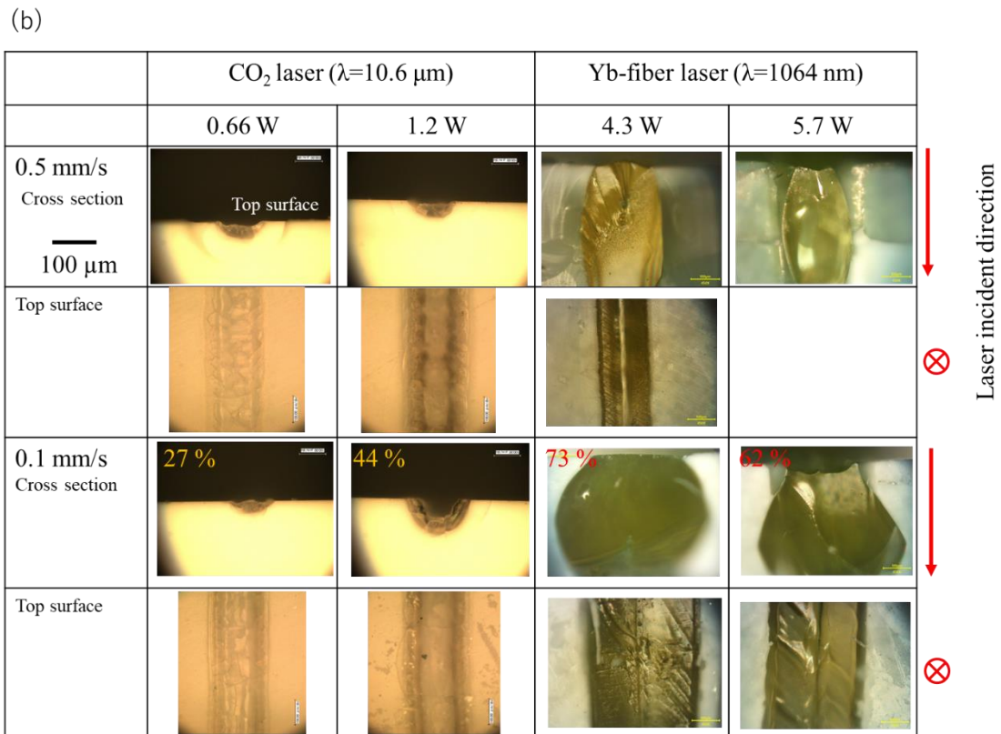
Figure 2.6(a) Schematic showing laser scan direction and cut line for cross section observation. (b) The cross-section image of laser irradiated glass plate with CO 2 laser (left 2 columns) and Yb-fiber laser (right 2 columns).
