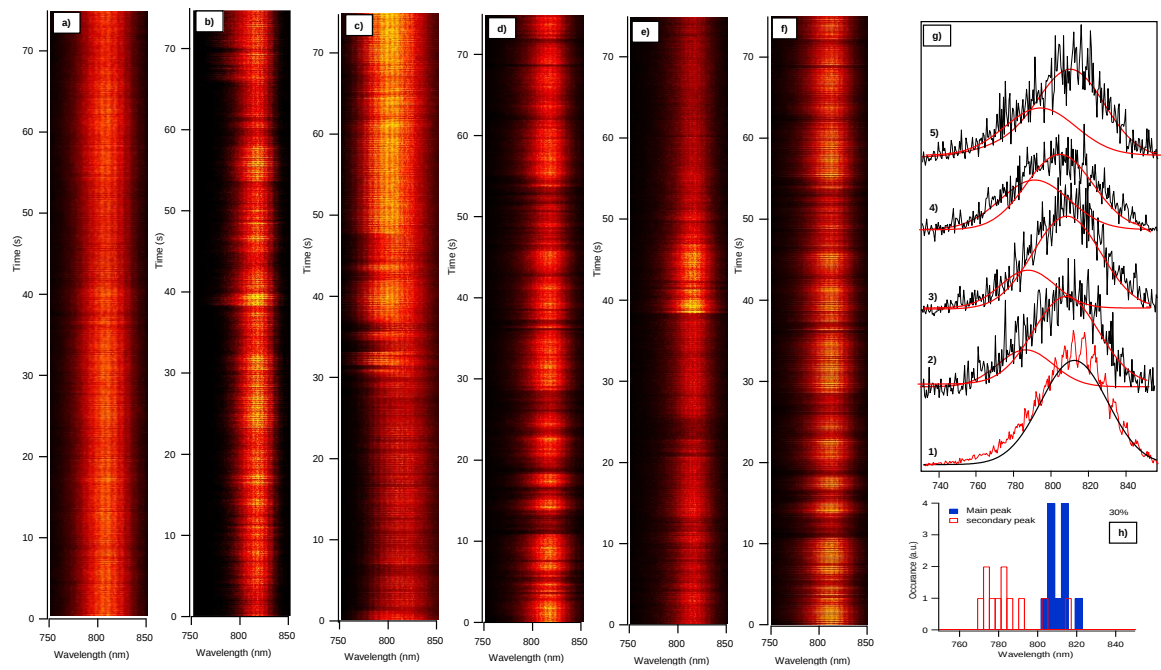
Figure 5.9. Time evolution PL Spectra of \text{MA}_{0.7}\text{FA}_{0.3}\text{PbI}_3 perovskite film. (a) PL spectra without external voltage. (b-f) PL spectra with applied 5V external voltage. (g) 2-4: PL spectra under applied field of 5V taken at different times from the trace (c); 1: PL spectrum without external field taken from the trace (a). The solid lines are Gaussian fits to the spectra. (h) Histogram of PL spectral peaks analyzed from the traces (b) - (f).
