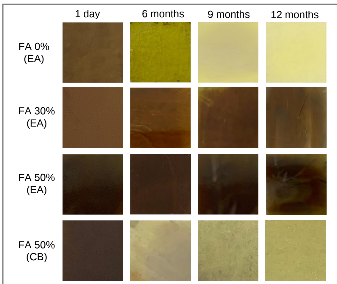
Figure 4.1. Photographs of perovskite films of prepared on 24 x 24 mm microscope cover glass at different stages of aging from 1 day to 12 months. The perovskite compositions and antisolvent used are indicated in the Figure (EA: Ethyl acetate).
