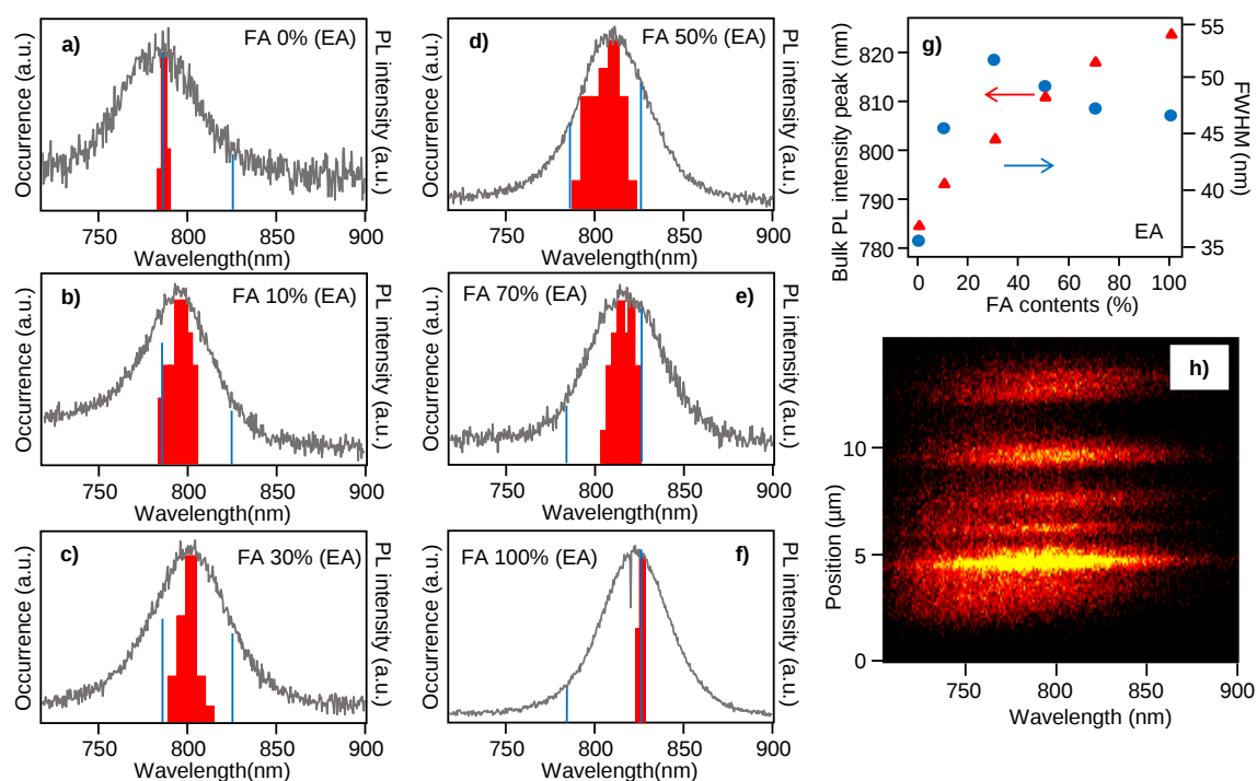
Figure 3.4. (a)-(f) Bulk PL spectra (solid grey lines) and histograms of local PL spectral maxima (red bars) for different compositions of films prepared using the EA antisolvent. The blue lines indicate the positions of the distribution peaks for FA 0% and FA 100% samples. (g) PL spectral maxima (red symbols) and FWHM (blue symbols) obtained from the bulk film PL spectra in (a)-(f) for the different compositions. (h) Example of 2D spectral plot (position vs. wavelength) for a selected location in the FA 30% film.
