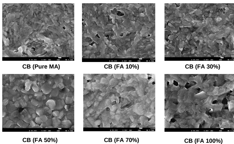
Figure 2.14. SEM images of \text{MA}_x\text{FA}_{1-x}\text{PbI}_3 for 1.0 M precursor solution
