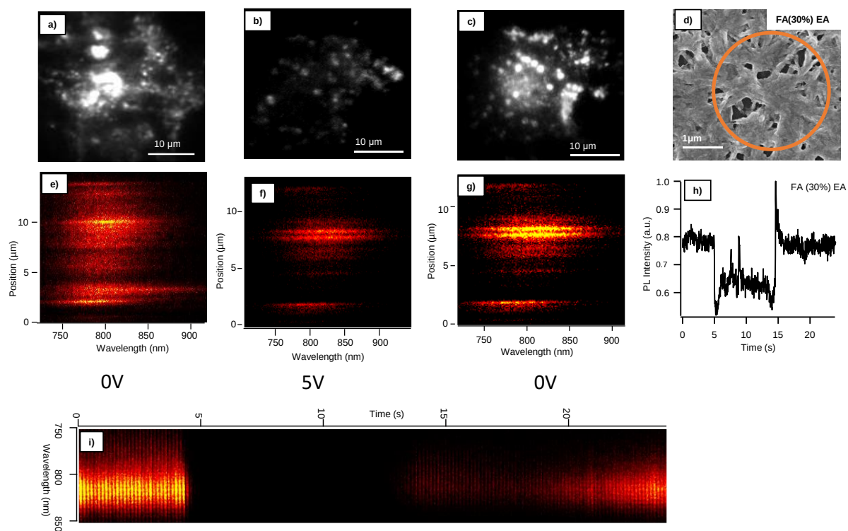
Figure 5.3. PL quenching and recovery of \text{MA}_{0.7}\text{FA}_{0.3}\text{PbI}_3 perovskite sample
