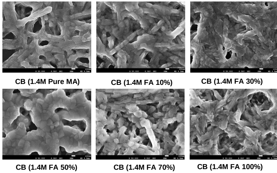
Figure 2.13. SEM images of \text{MA}_x\text{FA}_{1-x}\text{PbI}_3 for 1.4M precursor solution
