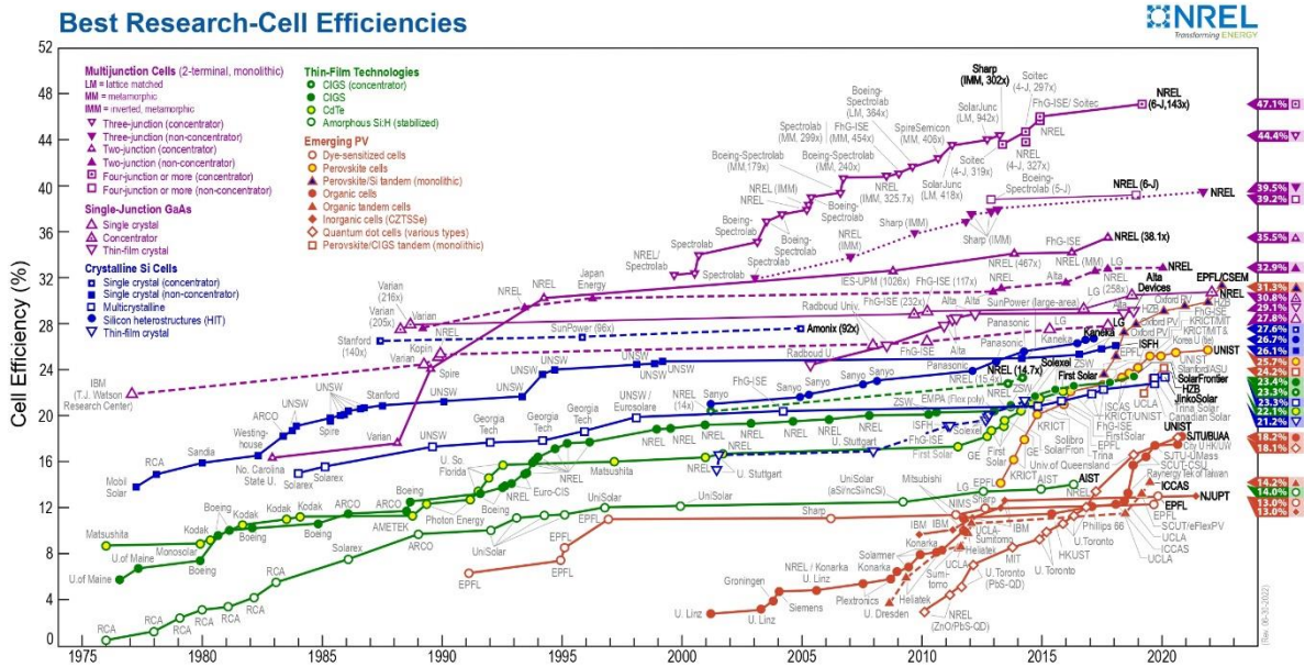
Figure 1.2. NREL chart of the highest confirmed conversion efficiencies for research cells for a range of photovoltaic technologies, plotted from 1976 to the present (reproduced with ref. 2 with permission).
