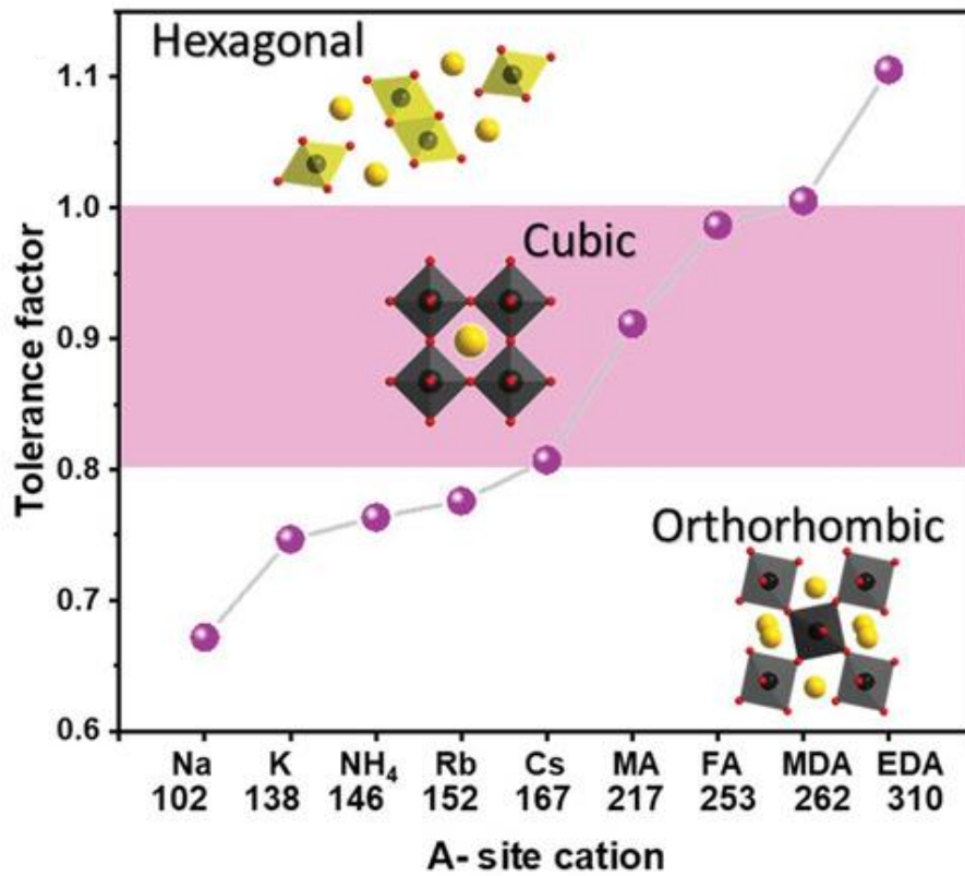
Figure 2.1. Dependency of tolerance factor of \text{APbI}_3 perovskites depending on A-cation radius. Colored part means region for stable cubic structure ( 0.8 < t < 1 ) (reproduced from ref. 1 with permission).
