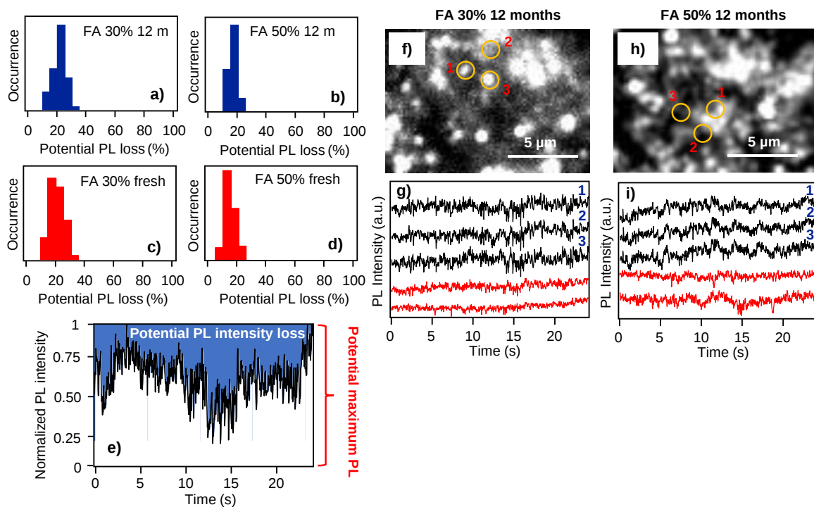
Figure 4.11. (a), (b) Histograms of the potential PL intensity loss obtained from PL blinking traces measured 12 months after film preparation, for sample compositions as indicated in the Figure. (c), (d) Same for freshly prepared films. (e) Example of a PL blinking trace
