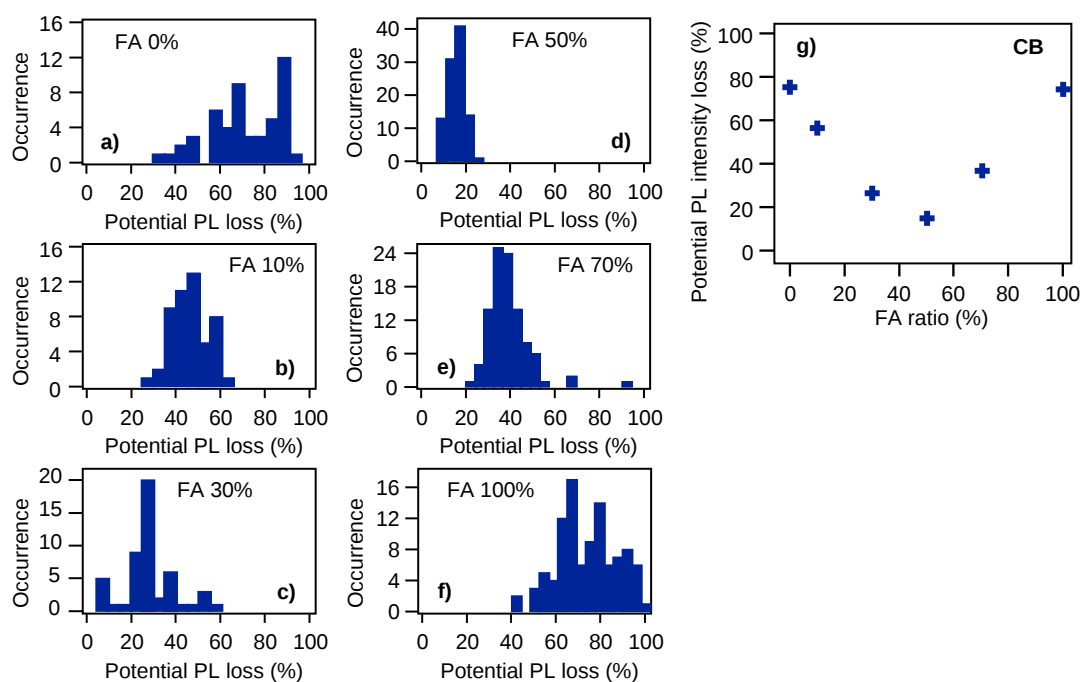
Figure 3.11. (a)-(f) Histograms of the potential PL intensity loss obtained for different film compositions prepared using the CB antisolvent. (g) Peaks of the distributions in (a)-(f) are plotted as a function of the FA content.
