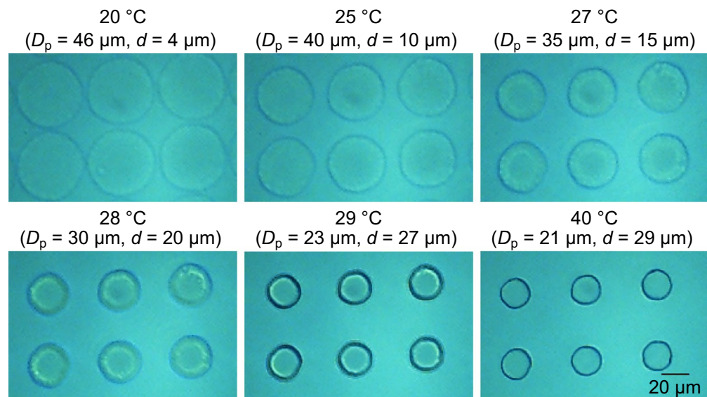
Figure 4. Top-view photomicrographs of the PNIPAM micropillars confined in the PDMS microchannel filled with the aqueous solution at different temperatures.
