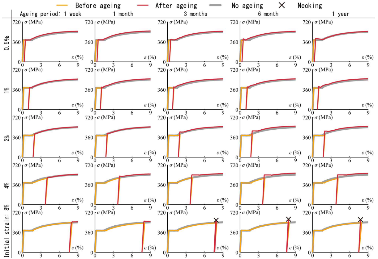
Figure 4: Representative stress-strain curves for reinforcement (SD345, D19) subjected to different initial tensile strain and ageing periods.
