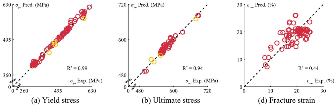
Figure 6: Verification of proposed models against experimental data.
