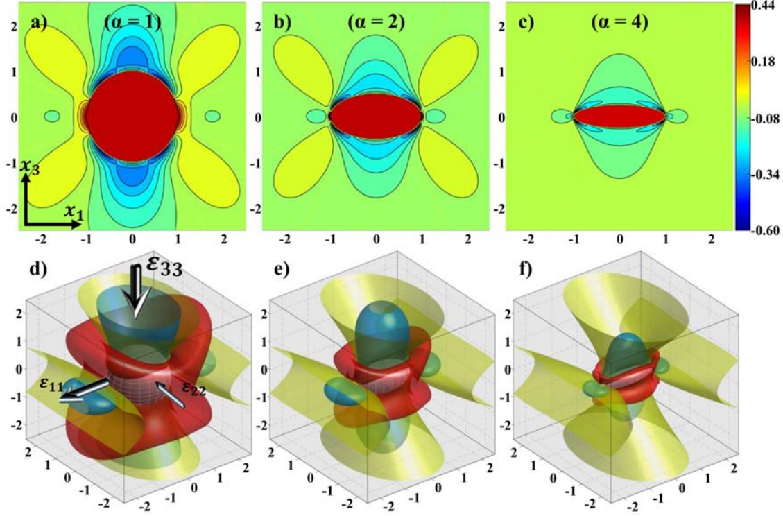
Figure 4.6: Strain disturbance, \tilde{\varepsilon}_{33} , around the inhomogeneity under cold rolling conditions for an aspect ratio of \alpha = 1.0 (a, d), 2.0 (b, e), or 4.0 (c, f).
