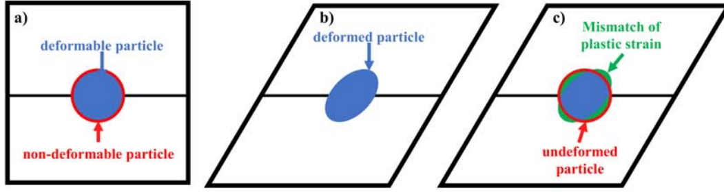
Figure 1.5: The incompatibility between a deformable matrix and a non-deformable particle. (a) Undeformed state, (b) with deformed particle, (c) with undeformed particle
