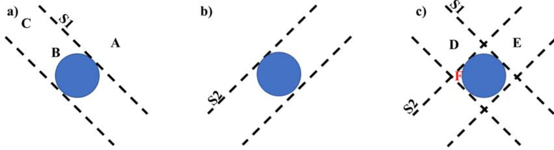
Figure 1.8: Schematic diagram of the slip shadowing model for the deformation zone. (a) Slip on system S_1 is restricted by the particle, (b) Slip on system S_2 is restricted by the particle, (c) Slip restriction on both systems S_1 and S_2 ( Humphreys and Ardakani, 1994 )
