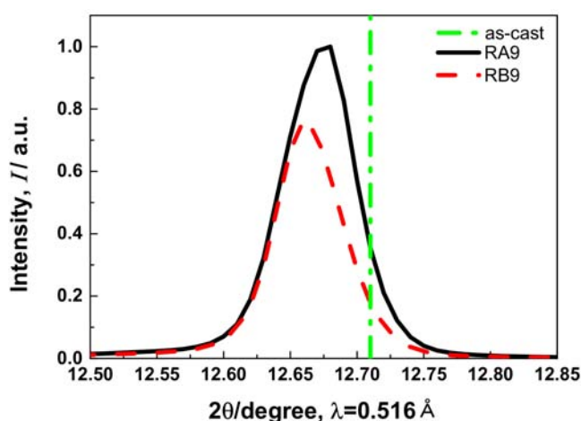
Figure 3.3: (111) diffracted peak at different homogenization condition for the RA9 and RB9
