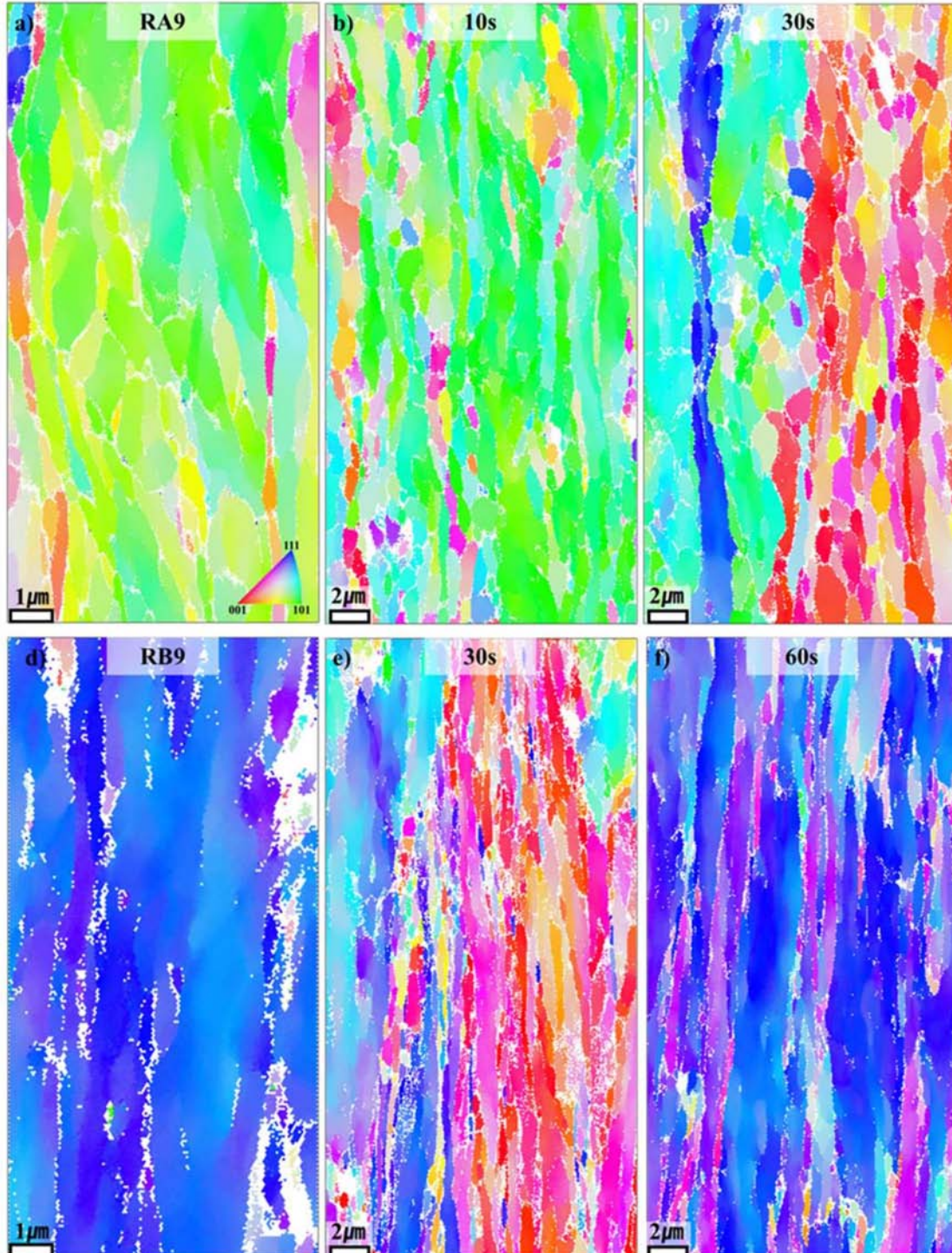
Figure 3.7: EBSD map in longitudinal section of (a-c) RA9 and (d-f) RB9 from cold-rolled state to the near point where recovery behavior ends during annealing at 280 °C. The inverse pole figures (IPF) indicate the color key of the crystal direction parallel to the normal direction (ND)
