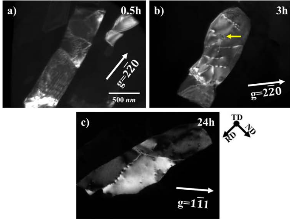
Figure 3.8: Microstructure evolution of the RA9 annealed at 220 °C for (a) 0.5h, (b) 3h and (c) 24h
