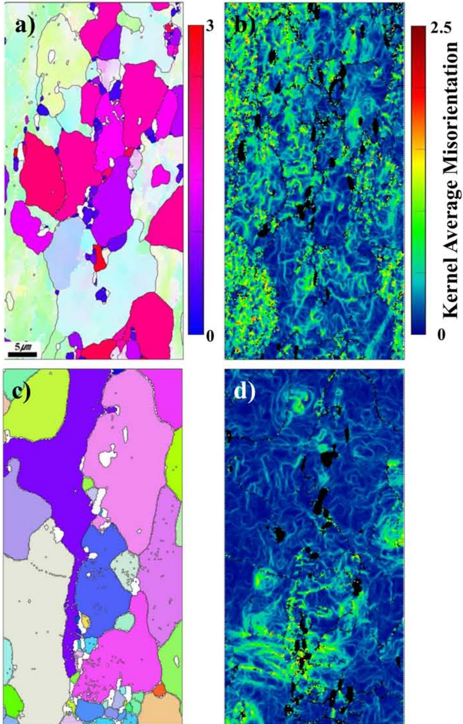
Figure 3.13: (a) Grain orientation spread (GOS) map overlaid with IPF map, (b, d) kernel average misorientation to the 1st neighbor with 2.5° threshold angle and (c) grain map in RB9 annealed at 350 °C for (a, b) 100s and (c, d) 1000s
