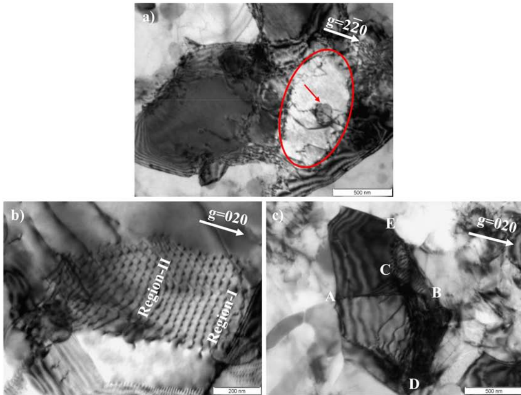
Figure 5.11: Evolution microstructure of AM5 annealed at 300 °C for (a) 120s and (b, c) 600s
