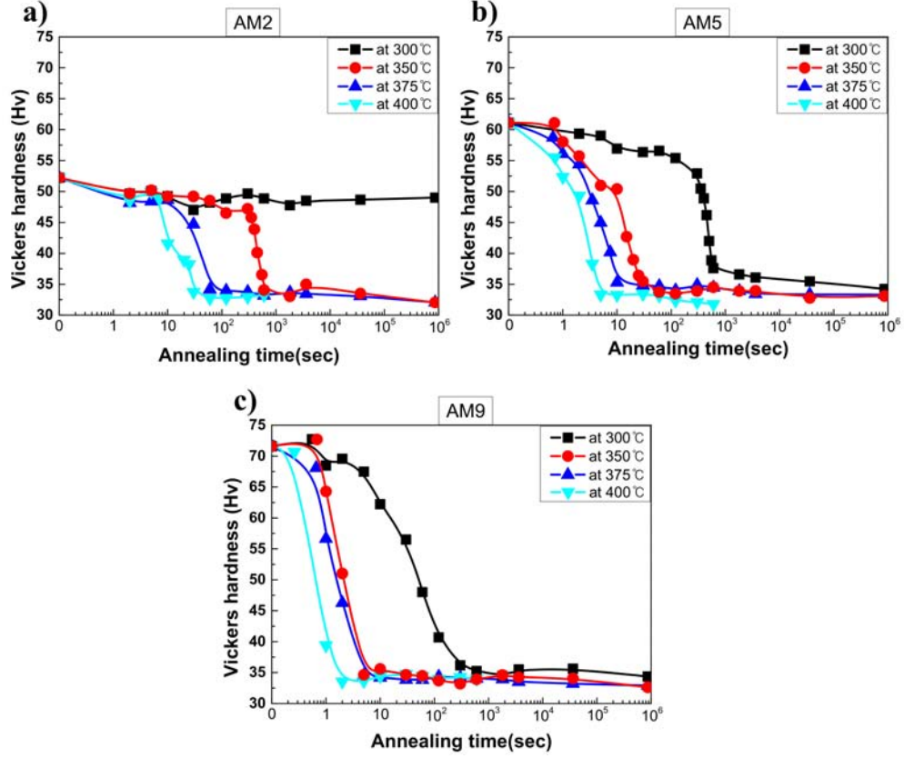
Figure 2.7: Relationship between Vickers hardness and the annealing time at each temperature of AM2, AM5 and AM9
