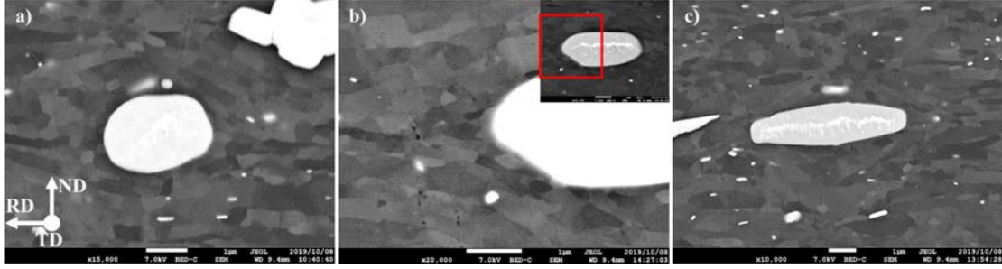
Figure 4.1: Micrograph showing a deformation zone around an \alpha -Al(Mn, Fe)Si particle with an aspect ratio of approximately (a) 1.0, (b) 2.0 or (c) 4.0 formed during cold rolling in the AA3003 aluminum alloy. The nominal strain of the cold rolled specimen is assumed to be 0.9.
