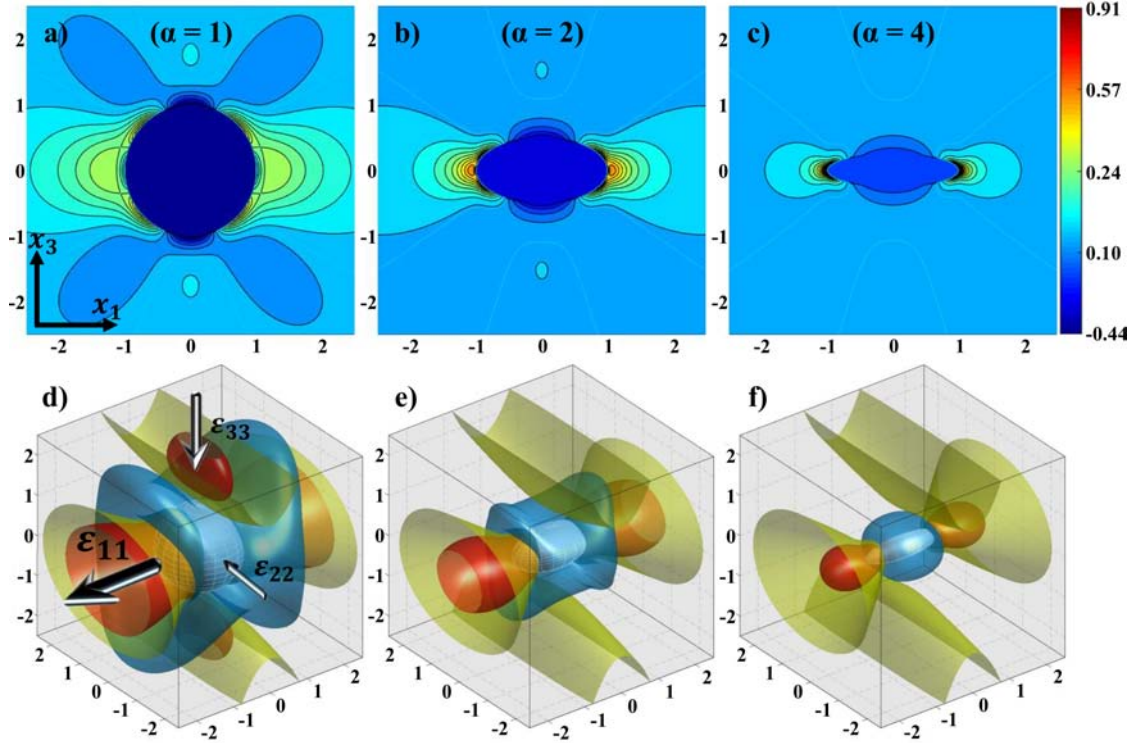
Figure 4.5: Strain disturbance, \tilde{\varepsilon}_{11} , around an inhomogeneity under cold rolling conditions for an aspect ratio of \alpha = 1.0 (a, d), 2.0 (b, e), or 4.0 (c, f).
