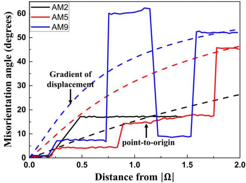
Figure 5.17: Misorientation angles profile across the rotated zone formed around the \alpha -Al(Mn, Fe)Si precipitate measured by prediction of displacement gradient and EBSD analysis.
