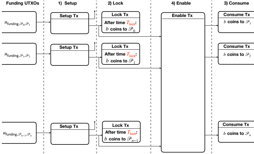
Figure 5.1: Informal illustration of AMCU as a transaction-tree.
