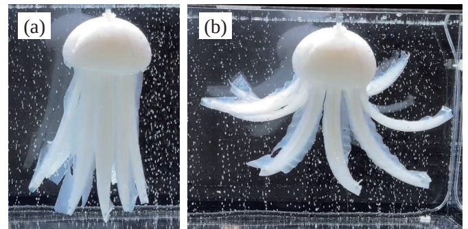
Fig.6 (a) The jellyfish healing robot when no air pressure is applied. (b) The jellyfish healing robot when 0.15 MPa air pressure is applied.
