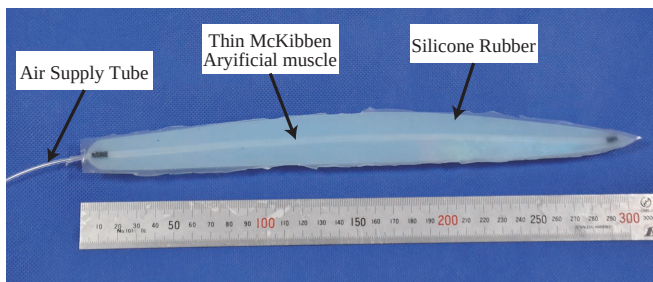
Fig.1 The leg of the jellyfish healing robot embedded with thin McKibben artificial musclesl.
