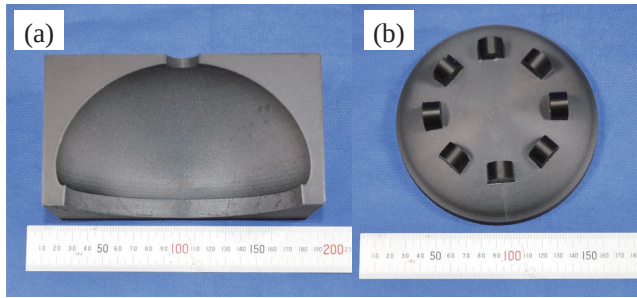
Fig.3 (a) The mold for producing head shape silicone rubber. (b) The mold for grooving the bottom of the head.
