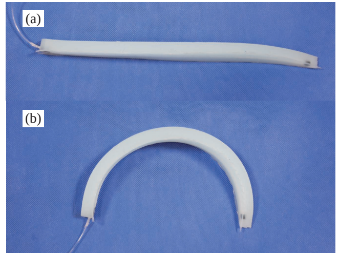
Fig.5 (a) The leg when no air pressure is applied. (b) The leg when 0.3 MPa air pressure is applied.
