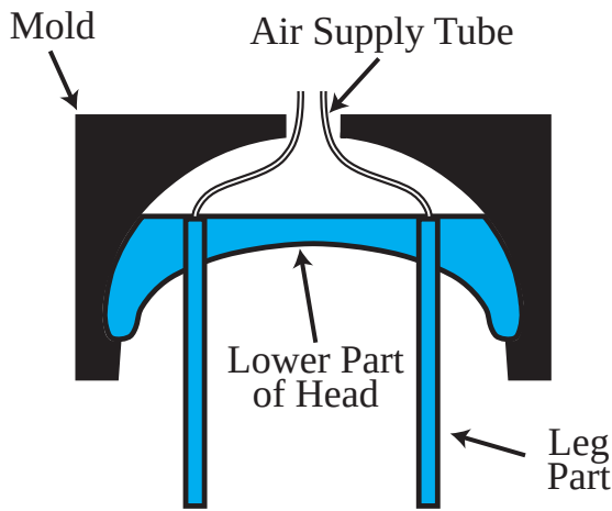
Fig.4 The Process of making the upper half of the head.
