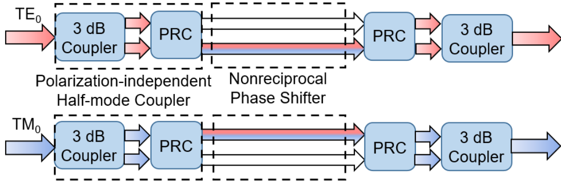
Fig.5-3 Mode conversion of the device under TE- and TM-polarized input.
