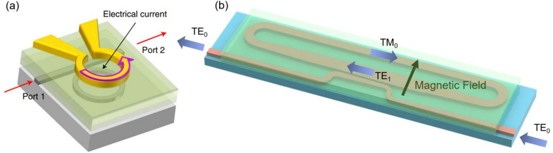
Fig. 4-2 (a) MRR nonreciprocal device fabricated by wafer bonding, the radial magnetic field was integrated by Au wires [5]. (b) The novel MRR nonreciprocal device fabricated by wafer bonding under a unidirectional magnetic field.
