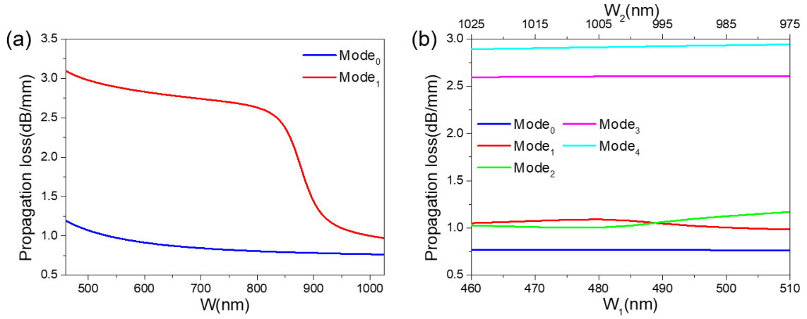
Fig.5-11 Mode propagation losses in (a) a single MO waveguide and (b) the coupler varies with waveguide width.
