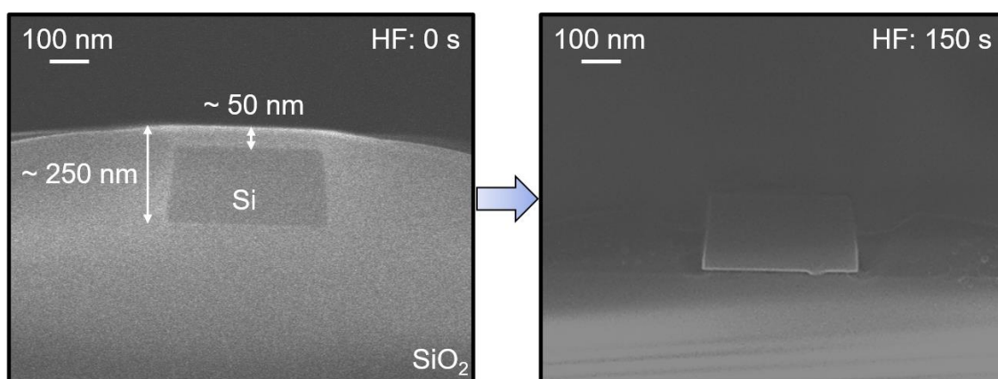
Fig. 4-11 SEM photos of the cross-section of the MO material integration window of the external-fab chip, (a) untreated and (b) HF solution wet etching for 150 s.
