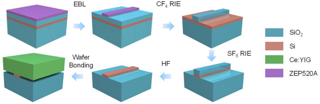
Fig.3-6 Process flow.
