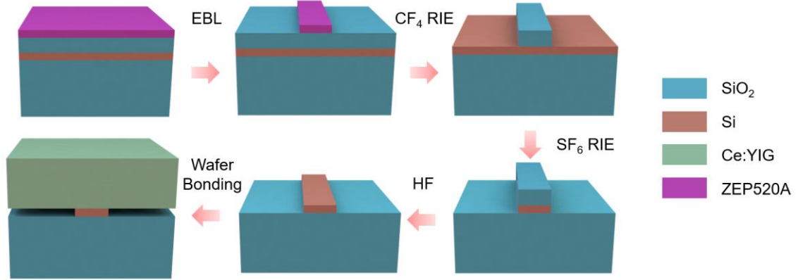
Fig. 4-6 Processing flow.
