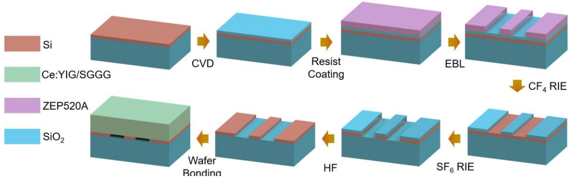
Fig.5-7 Processing flow.
