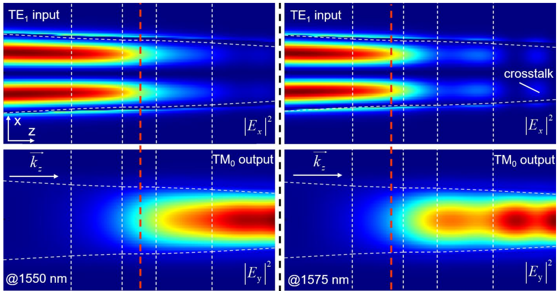
Fig.2-5 Transmission field distribution of TE 1 &TM 0 mode converters with nonlinear tapered waveguide at wavelengths of 1550 nm and 1575 nm.
