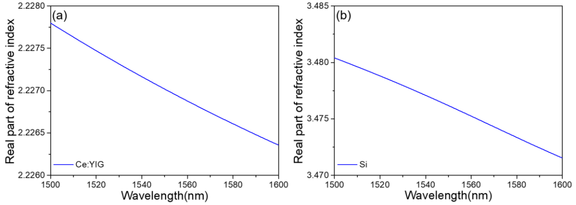
Fig.A1 Real part dispersion of refractive index of (a) Ce:YIG and (b) Si.
