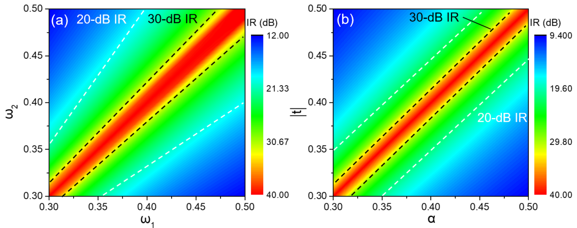
Fig.6-2 (a) The IR of MMI-type devices varies with the amplitude of the two modes for interference. (b) The relationship between IR and |t| and \alpha of MRR-type devices.
