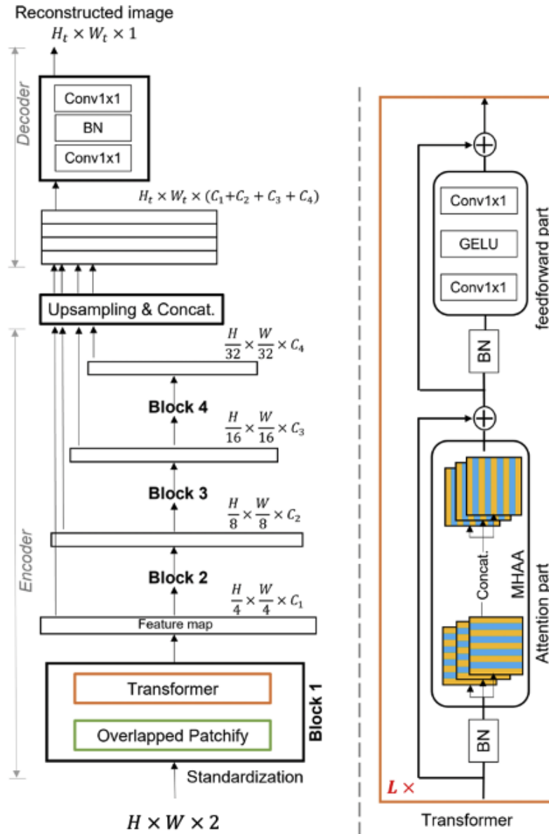
Fig. 4.5 Image reconstruction model. Revised from [53].
