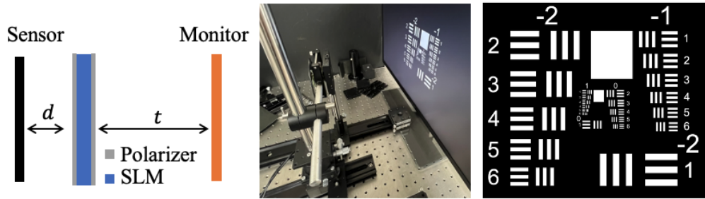
Fig. 3.13 Experiment setup and the resolution chart target.
