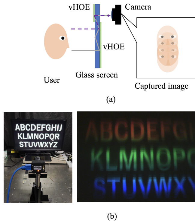
Fig. 5.3 Applications of HWD-based STS camera (a) Under-display-camera for a full-screen smartphone (b) near-screen touchless display.
