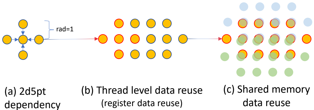
Figure 5.1: Spatial Blocking, using 2D 5-point Jacobian (2d5pt) stencil as an example
