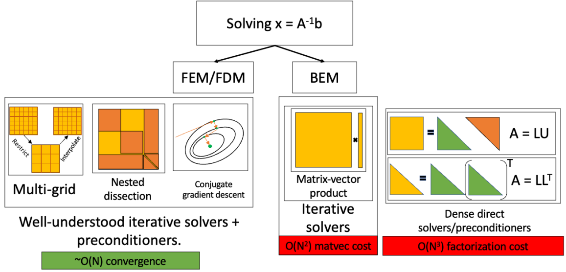
Figure 2.7: Various solvers proposed in the literature for sparse matrices arising out of FEM and FDM, and dense matrices arising out of BEM. Obtaining the solution to the system of linear equations such as Ax = b is at the heart of scientific computing.
