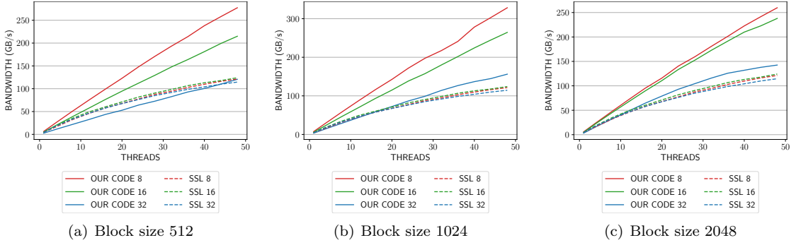
Figure 4.6: Bandwidth utilization for varying ranks and block sizes on Fujitsu A64FX. The legend shows the rank for each plot. The bandwidth is calculated using Eq. 4.3. The peak STREAM TRIAD bandwidth for the A64FX is about 840 GB/s.
