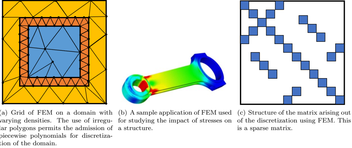
Figure 2.4: The grid resulting from FEM for a sample application. The rightmost figure shows the structure of the resulting stiffness matrix.
