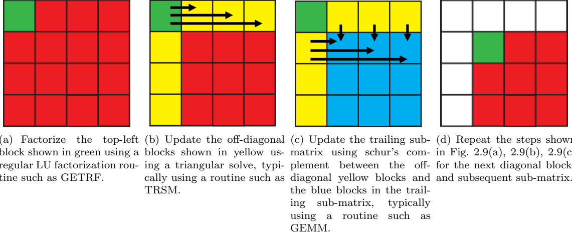
Figure 2.9: Steps of the block LU factorization algorithm without pivoting.
