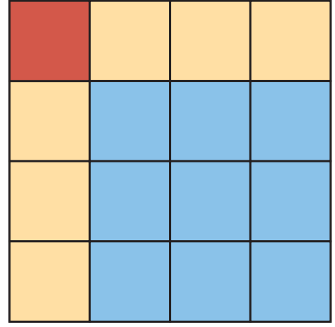
(b) Right looking block LU factorization.
