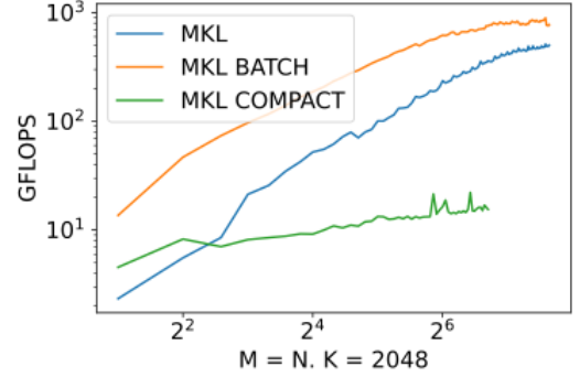
(b) Batched skinny matrix computation.
