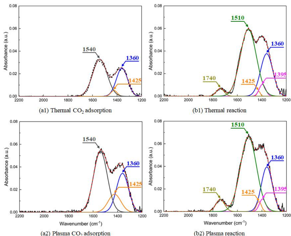
Figure 2.7 In situ DRIFTS spectra at 300 °C of CO 2 adsorption: (a1) thermal and (a2) plasma. CO 2 methanation: (b1) thermal and (b2) plasma. Monodentate carbonate ( 1360 and 1425\text{ cm}^{-1} ); Bidentate carbonate ( 1540\text{ cm}^{-1} ); Polydentate carbonate ( 1395 and 1510\text{ cm}^{-1} ); Formyl ( 1740\text{ cm}^{-1} ).
