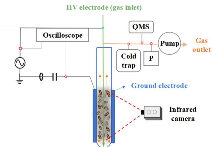
Figure 3.1 Experimental system of auto-methanation.
