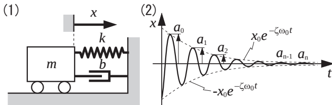
Fig.1 Simplified model and peak of damping vibration
