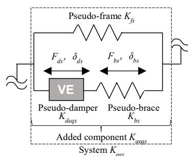
Fig.3 Shear model
