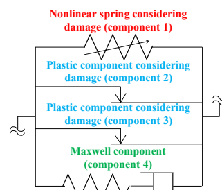
Fig.2 Analytical model of viscoelastic damper
