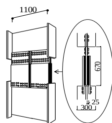
Fig.1 Stud-type viscoelastic damper [unit : mm]
